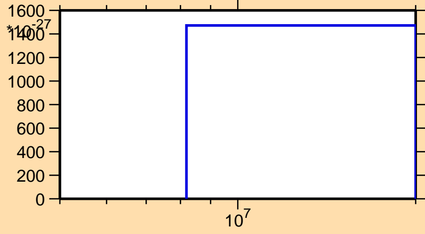
\sigma vs. E for ^{138}\text{Cs} (mt 42)
