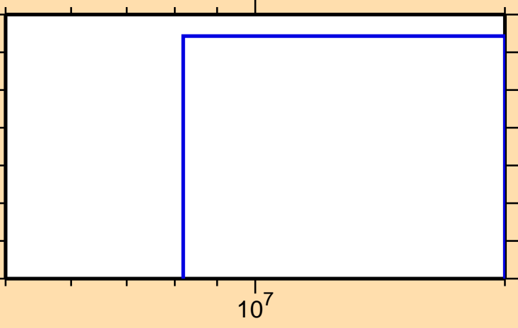
\sigma vs. E for ^{138}\text{Cs}(n,3n)
