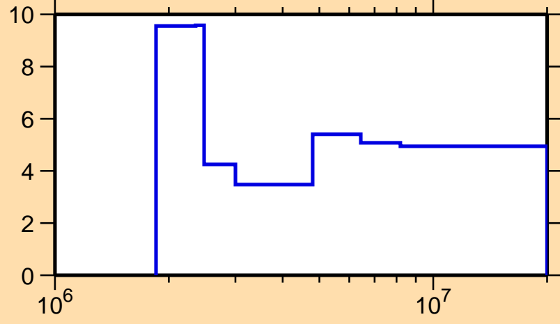
\Delta\sigma/\sigma vs. E for ^{138}\text{Cs}(n,n\text{onel.})
