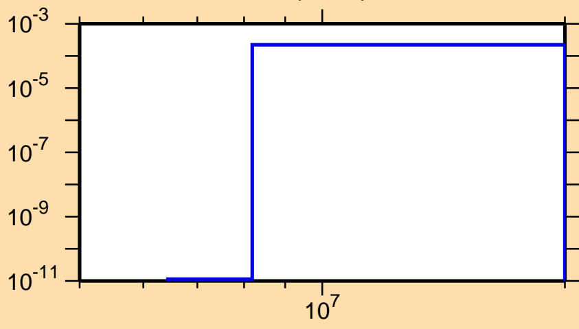
\sigma vs. E for ^{138}\text{Cs}(n,n\alpha)
