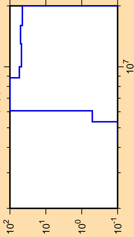
\Delta\sigma/\sigma vs. E for ^{139}\text{Cs}(n,p)
