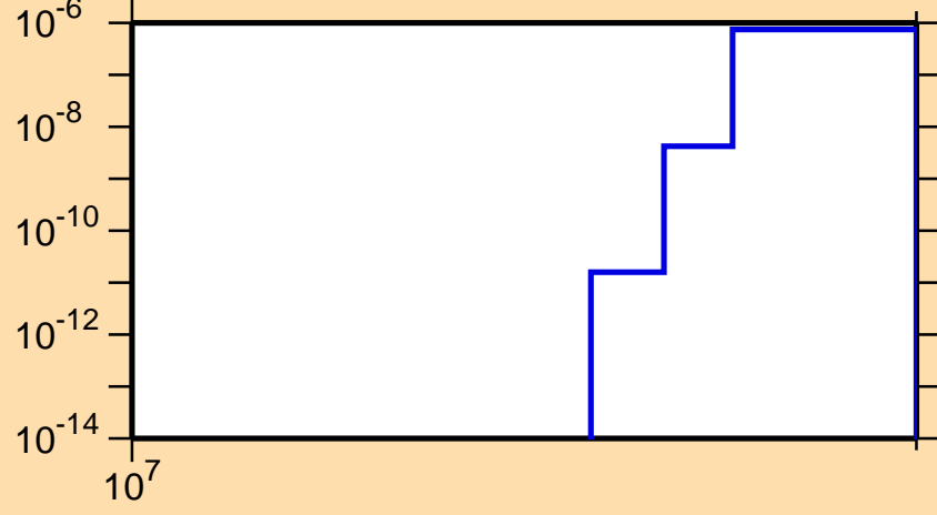
\sigma vs. E for ^{139}\text{Cs}(n,2np)
