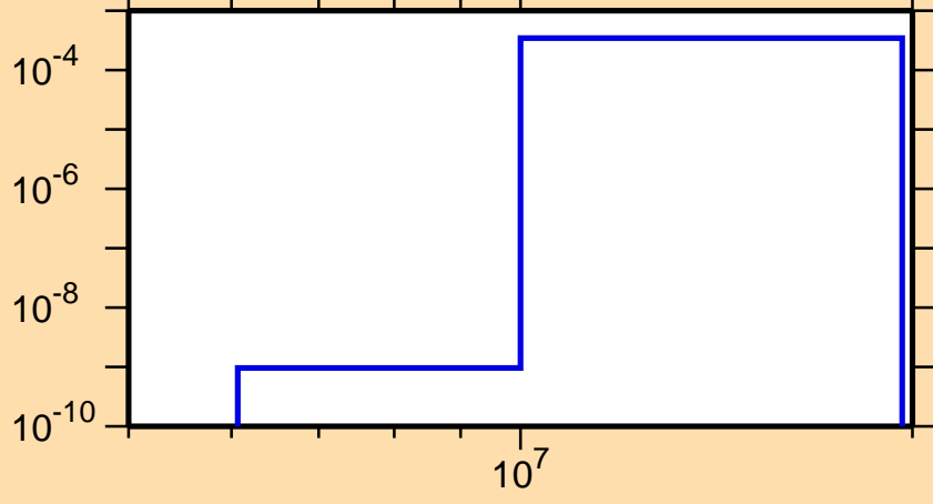
\sigma vs. E for ^{139}\text{Cs}(n,d)
