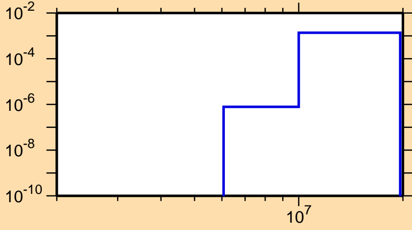
\sigma vs. E for ^{139}\text{Cs}(n,p)
