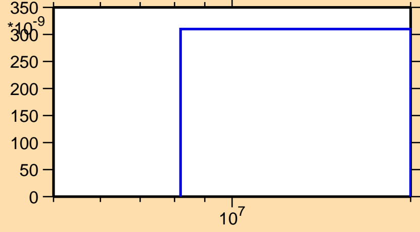
\sigma vs. E for ^{139}\text{Cs}(n,\text{nd})
