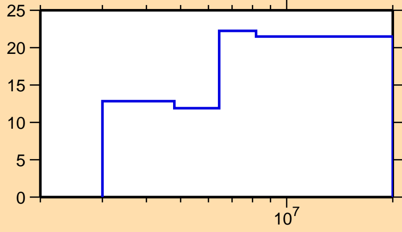
\Delta\sigma/\sigma vs. E for ^{139}\text{Cs}(n,ncont.)
