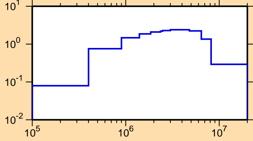
\sigma vs. E for ^{139}\text{Cs}(n,\text{inel.})
