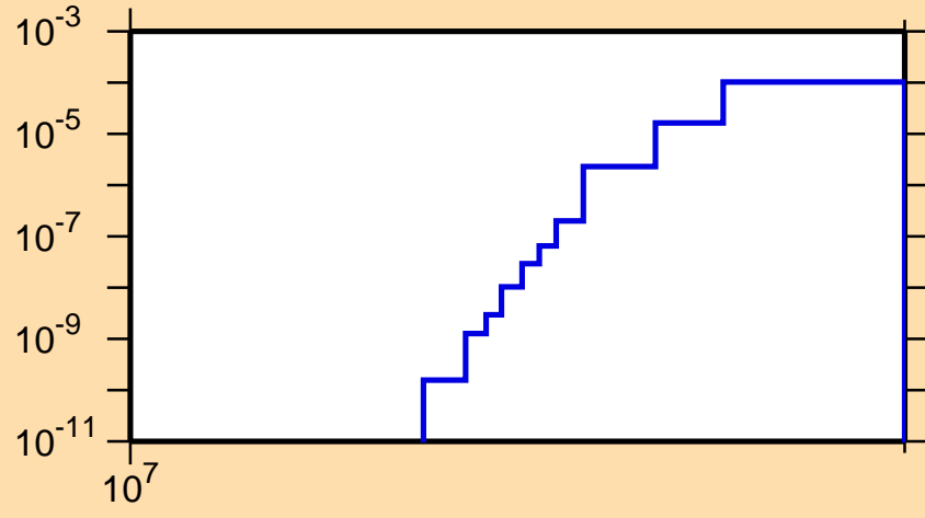
\sigma vs. E for ^{140}\text{Cs}(n,nd)
