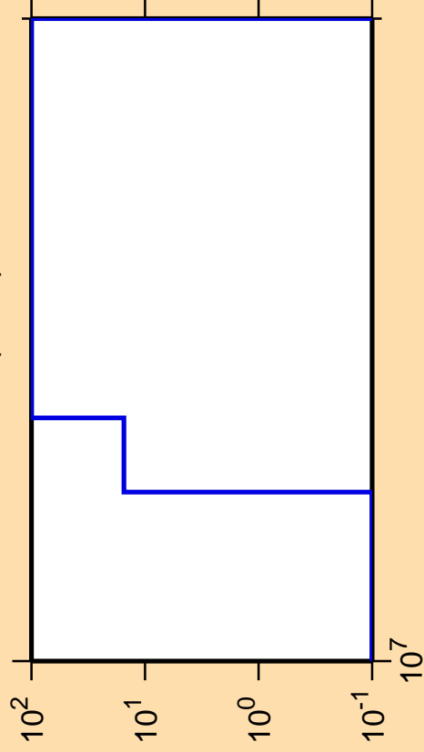
\Delta\sigma/\sigma vs. E for ^{140}\text{Cs}(n,nd)
