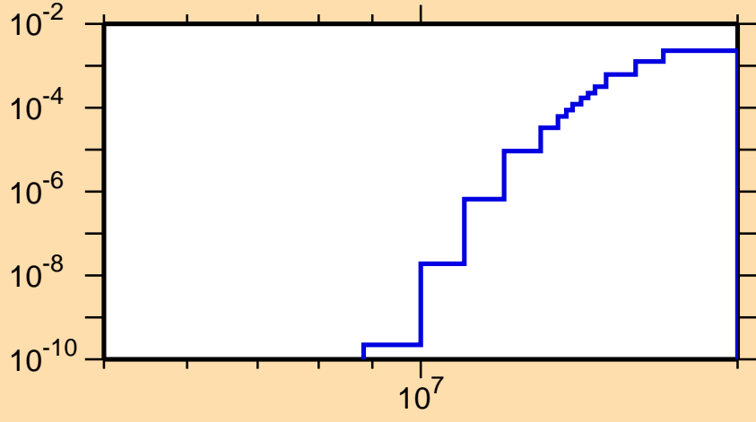
\sigma vs. E for ^{140}\text{Cs}(n,d)
