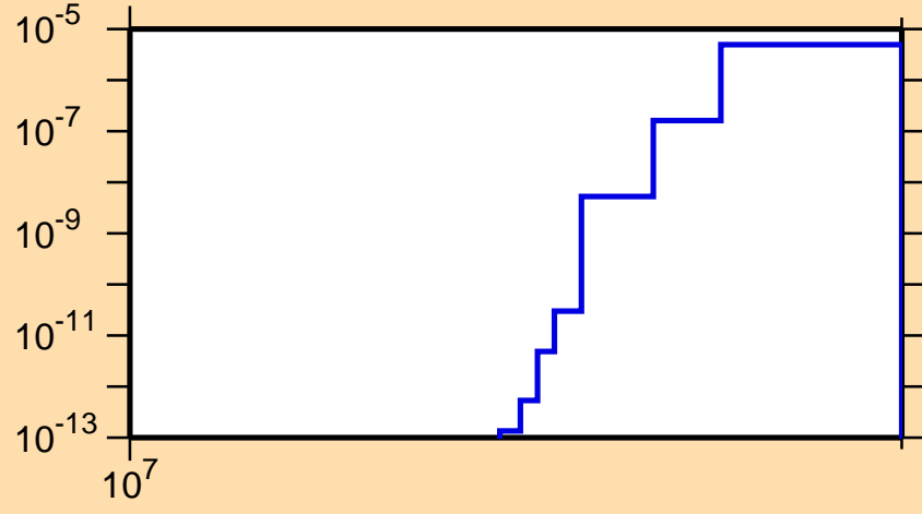
\sigma vs. E for ^{140}\text{Cs}(n,2np)
