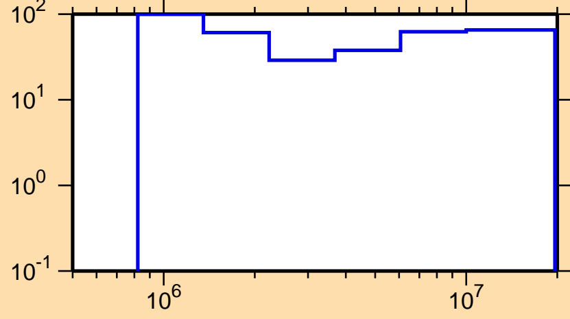
\Delta\sigma/\sigma vs. E for ^{140}\text{Cs}(n,n\text{cont.})
