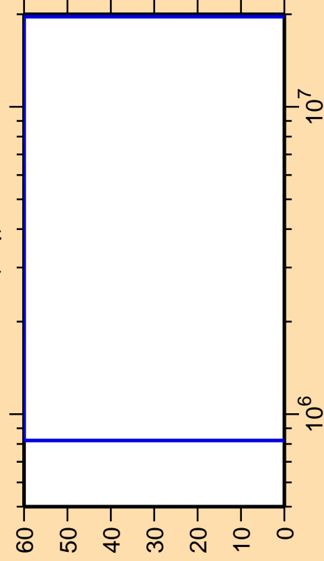
\Delta\sigma/\sigma vs. E for ^{140}\text{Cs}(n,\gamma)
