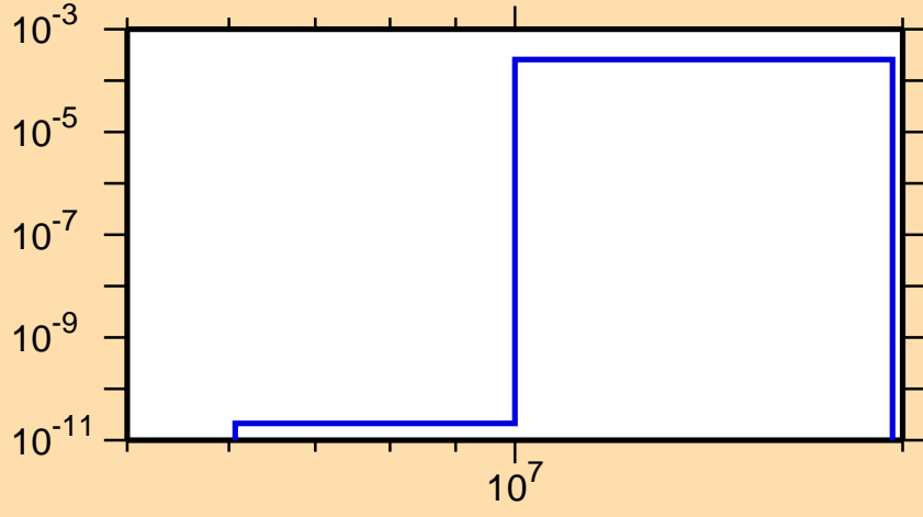
\sigma vs. E for ^{140}\text{Cs}(n,d)
