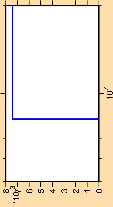
\Delta\sigma/\sigma vs. E for ^{140}\text{Cs}(n,3n\alpha)
