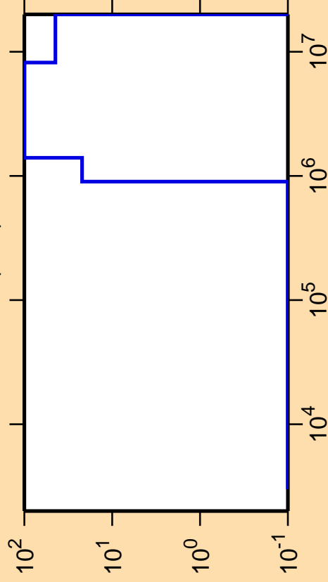
\Delta\sigma/\sigma vs. E for ^{140}\text{Cs}(n,\alpha)
