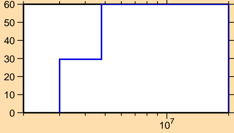
\Delta\sigma/\sigma vs. E for ^{140}\text{Cs}(n,ncont.)
