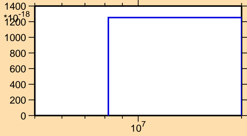
\sigma vs. E for ^{140}\text{Cs}(n,p\alpha)
