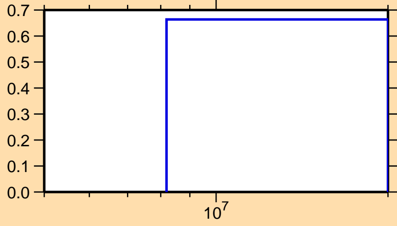
\sigma vs. E for ^{140}\text{Cs}(n,3n)
