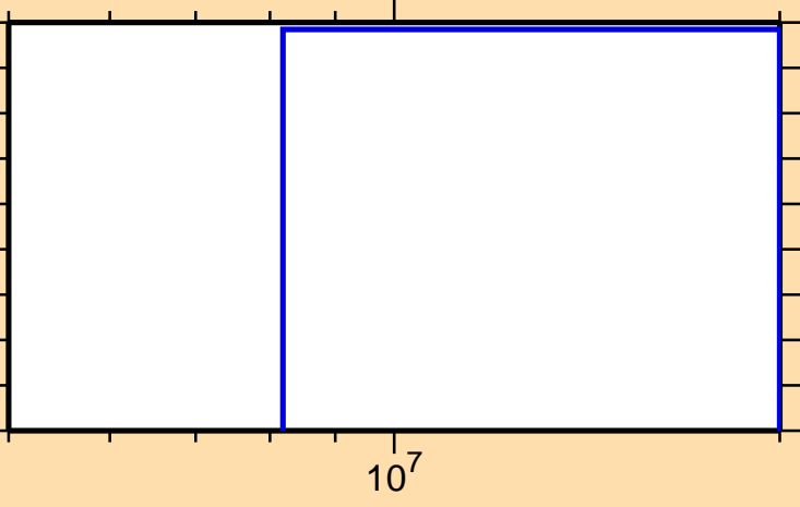
\sigma vs. E for ^{140}\text{Cs}(n,\text{nd})
