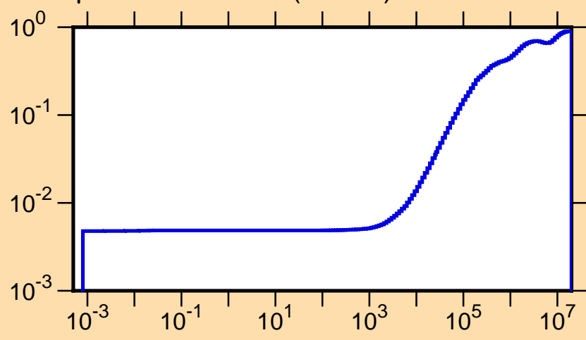
\mu vs. E for ^{141}\text{Cs}(\text{mt251})
