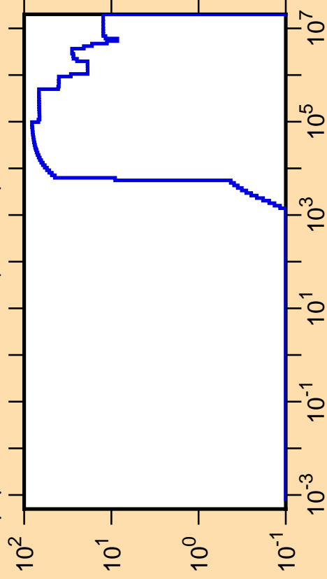
\Delta\mu/\mu vs. E for ^{141}\text{Cs}(\text{mt251})
