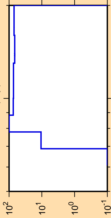
\Delta\sigma/\sigma vs. E for ^{141}\text{Cs}(n,p)
