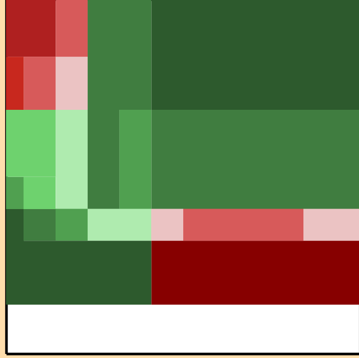
\Delta\sigma/\sigma vs. E for ^{141}\text{Cs}(n,n_1)
