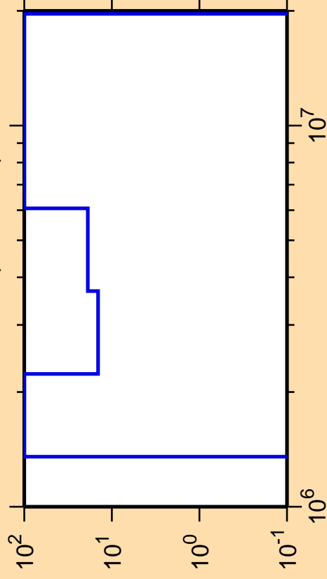
\Delta\sigma/\sigma vs. E for ^{141}\text{Cs}(n,ncont.)
