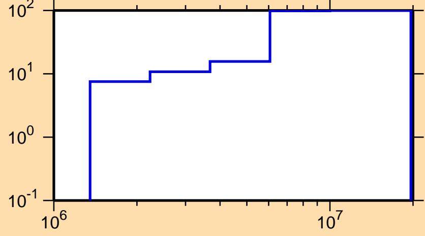
\Delta\sigma/\sigma vs. E for ^{141}\text{Cs}(n,inel.)
