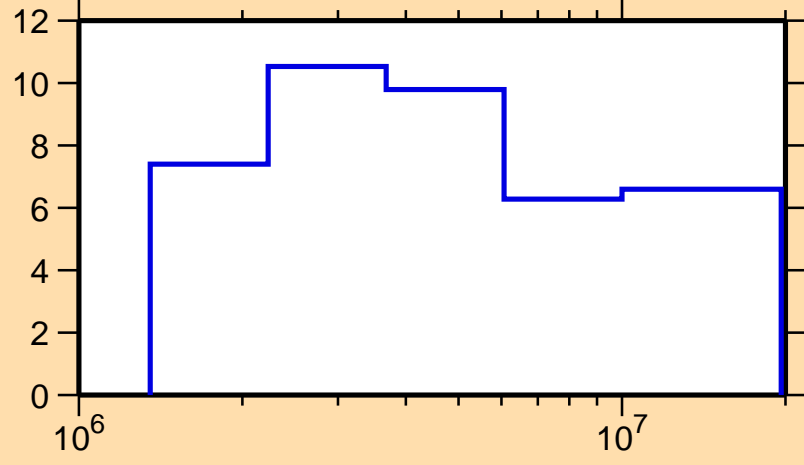
\Delta\sigma/\sigma vs. E for ^{141}\text{Cs}(n,n\text{onel.})
