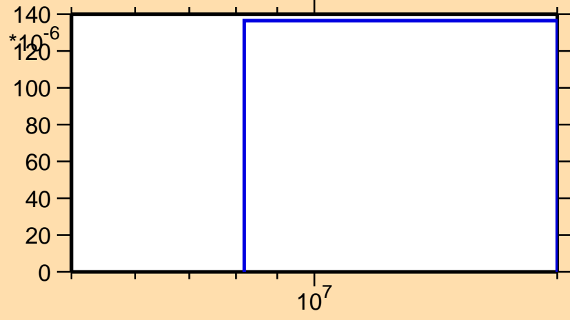
\sigma vs. E for ^{141}\text{Cs}(n,d)
