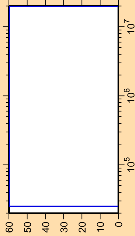
\Delta\sigma/\sigma vs. E for ^{141}\text{Cs}(n,\gamma)
