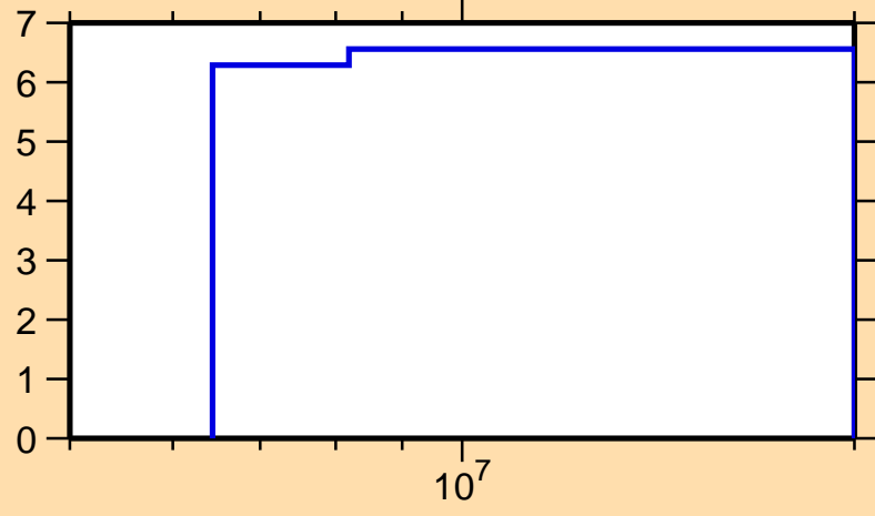
\Delta\sigma/\sigma vs. E for ^{141}\text{Cs}(n,\text{nonel.})
