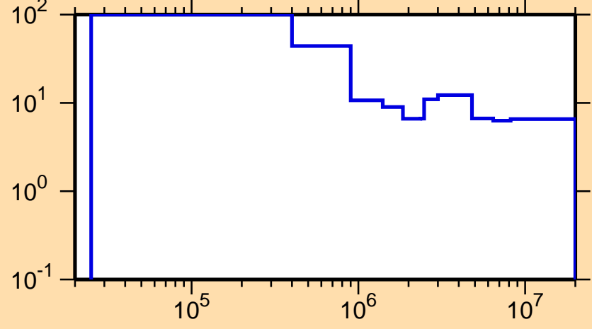
\Delta\sigma/\sigma vs. E for ^{141}\text{Cs}(n,\text{nonel.})
