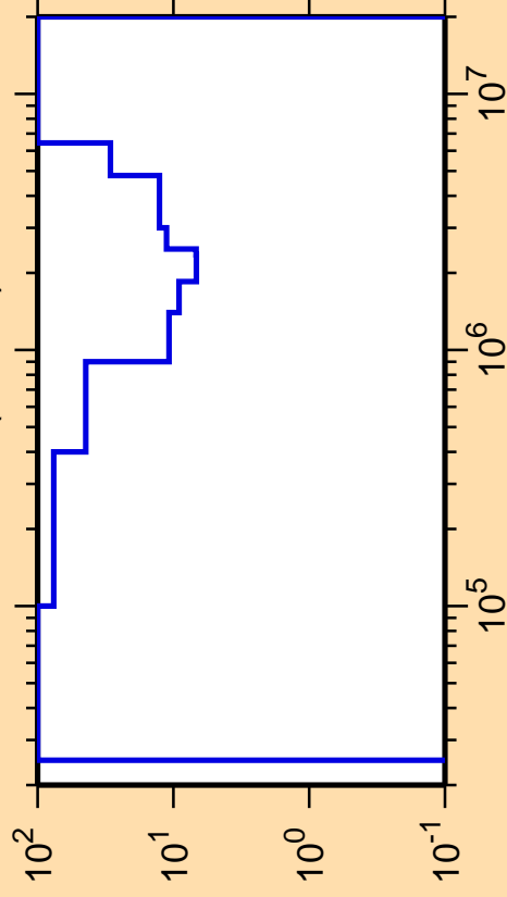
\Delta\sigma/\sigma vs. E for ^{141}\text{Cs}(n,\text{inel.})
