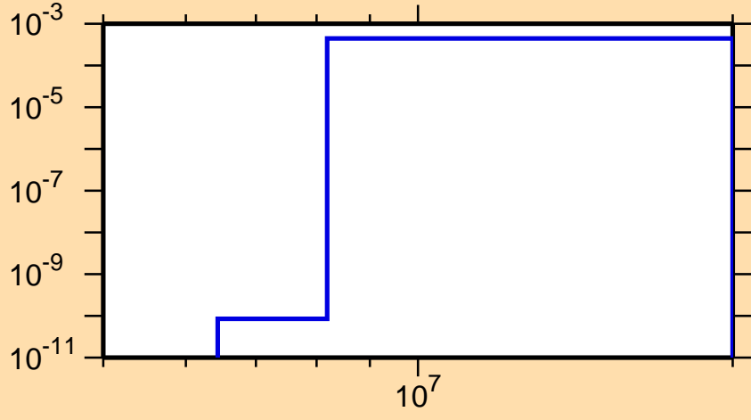
\sigma vs. E for ^{141}\text{Cs}(n,p)
