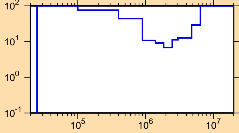
\Delta\sigma/\sigma vs. E for ^{141}\text{Cs}(n,\text{inel.})
