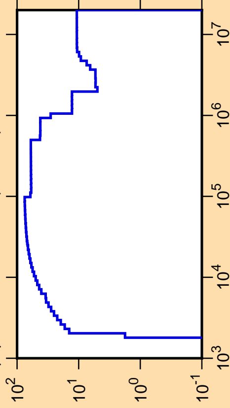
\Delta\mu/\mu vs. E for ^{142}\text{Cs}(\text{mt251})
