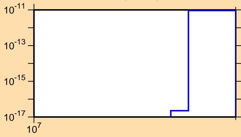
\sigma vs. E for ^{142}\text{Cs} (mt 11)
