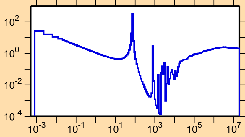
\sigma vs. E for ^{142}\text{Cs}(n,\text{nonel.})
