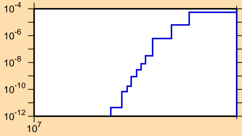
\sigma vs. E for ^{142}\text{Cs}(n,\text{nd})
