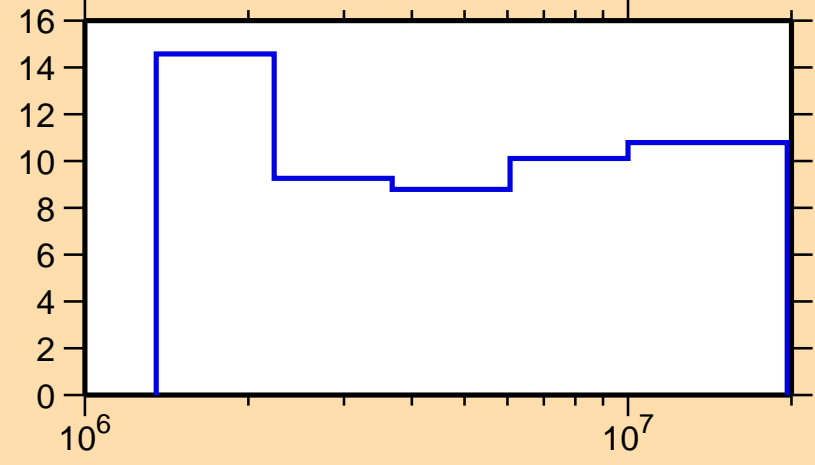
\Delta\sigma/\sigma vs. E for ^{142}\text{Cs}(n,n\text{onel.})
