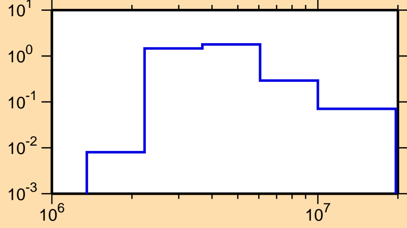
\sigma vs. E for ^{142}\text{Cs}(n,n\text{cont.})
