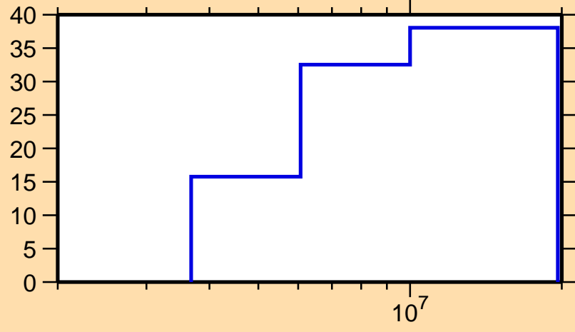
\Delta\sigma/\sigma vs. E for ^{142}\text{Cs}(n,ncont.)
