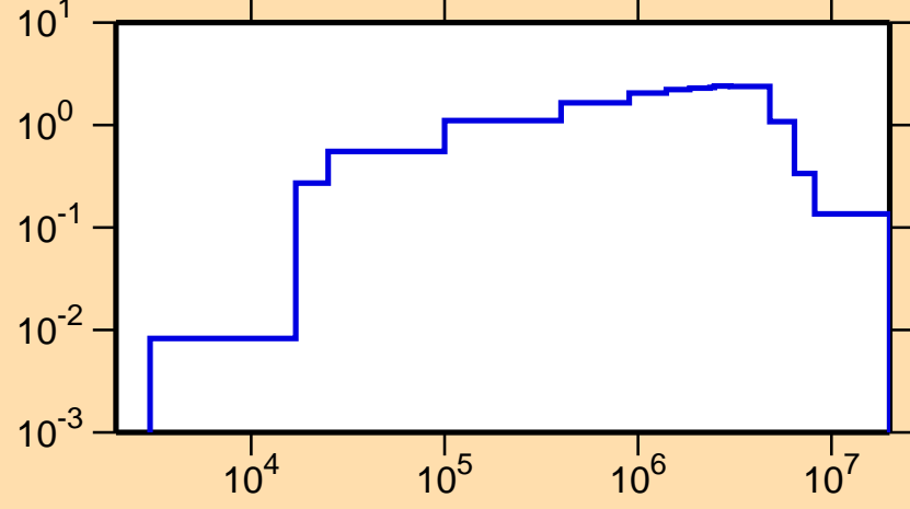
\sigma vs. E for ^{142}\text{Cs}(n,\text{inel.})
