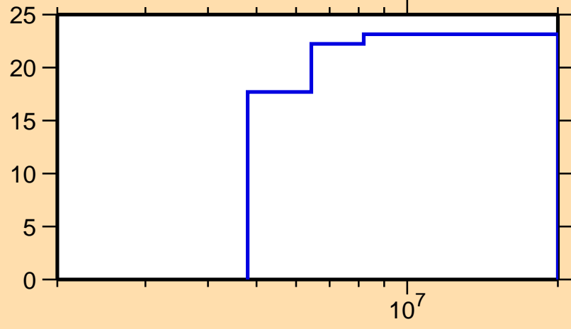
\Delta\sigma/\sigma vs. E for ^{142}\text{Cs}(n,\text{inel.})
