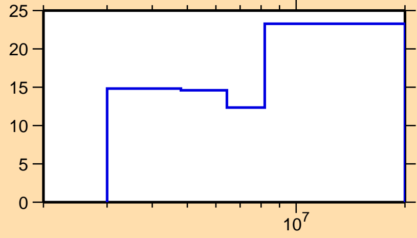
\Delta\sigma/\sigma vs. E for ^{142}\text{Cs}(n,2n)
