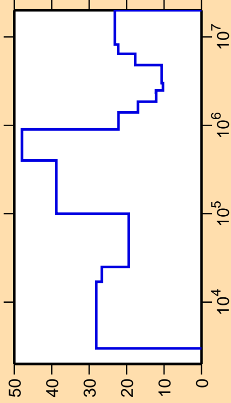
\Delta\sigma/\sigma vs. E for ^{142}\text{Cs}(n,\text{inel.})
