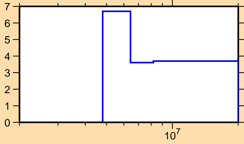
\Delta\sigma/\sigma vs. E for ^{142}\text{Cs}(n,\text{tot.})
