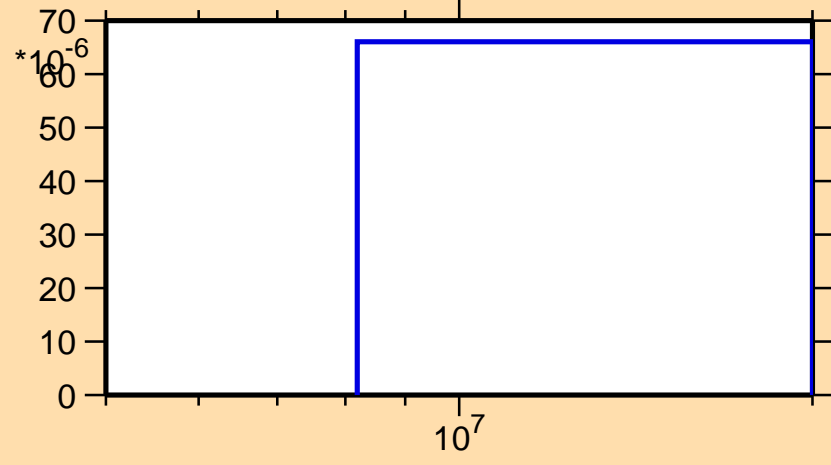
\sigma vs. E for ^{142}\text{Cs}(n,d)
