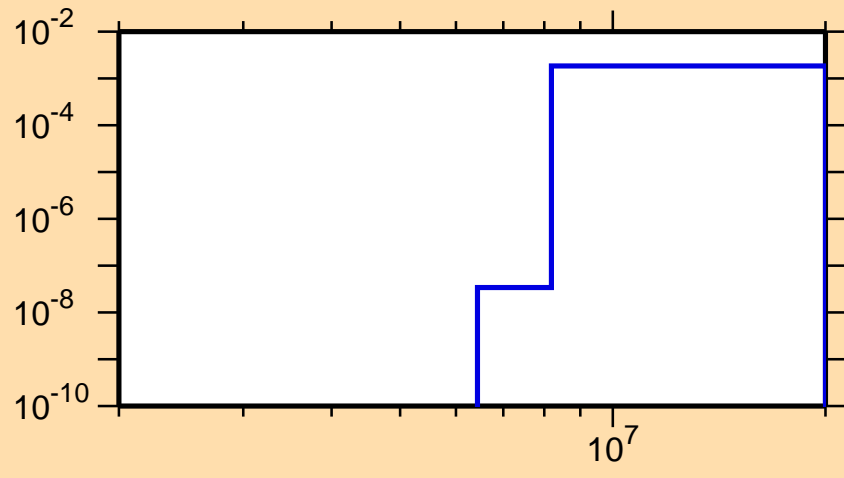
\sigma vs. E for ^{142}\text{Cs}(n,p)
