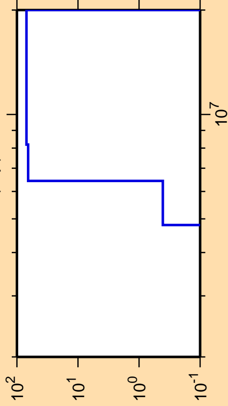
\Delta\sigma/\sigma vs. E for ^{142}\text{Cs}(n,p)
