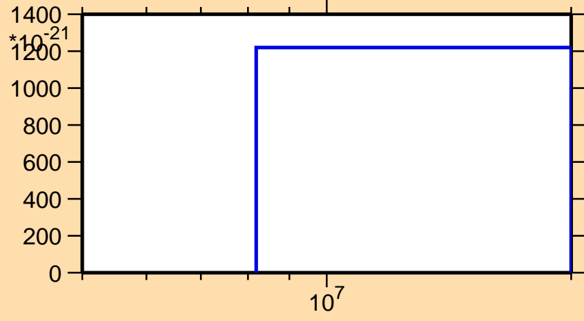
\sigma vs. E for ^{142}\text{Cs} (mt 42)
