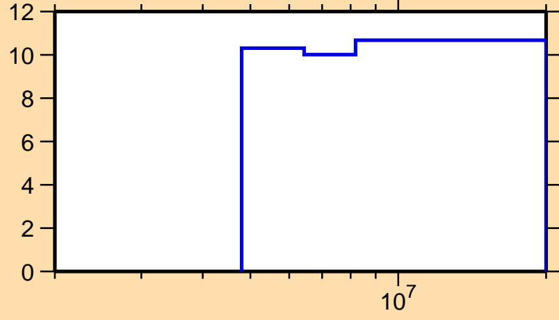
\Delta\sigma/\sigma vs. E for ^{142}\text{Cs}(n,\text{nonel.})
