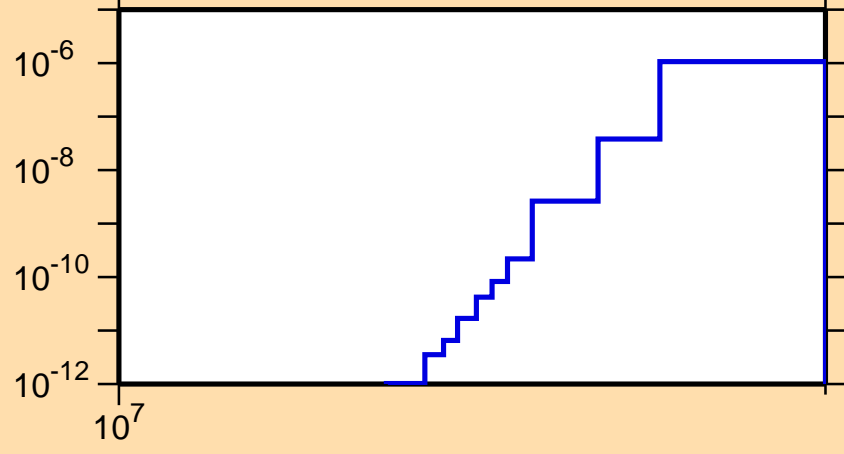
\sigma vs. E for ^{143}\text{Cs}(n,2n\alpha)
