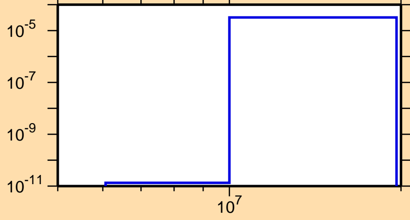
\sigma vs. E for ^{143}\text{Cs}(n,n\alpha)
