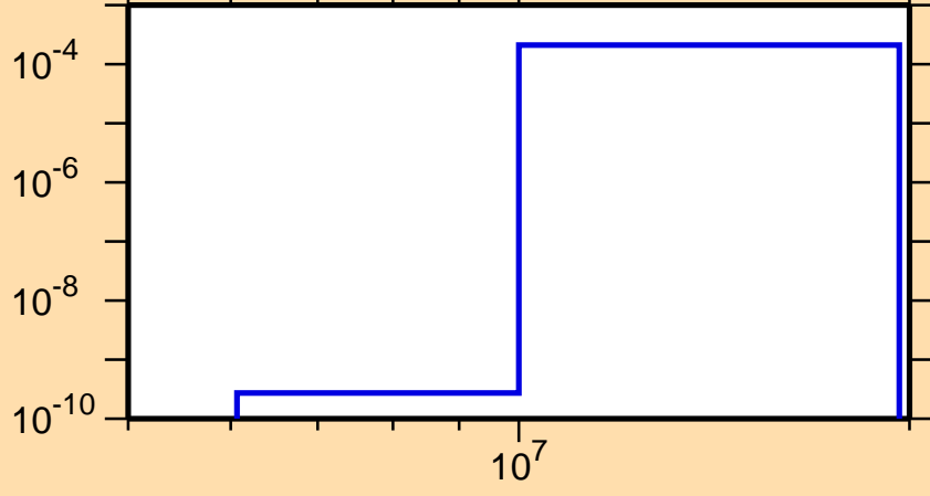
\sigma vs. E for ^{143}\text{Cs}(n,p)
