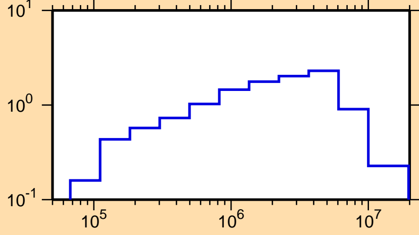
\sigma vs. E for ^{143}\text{Cs}(n,\text{inel.})
