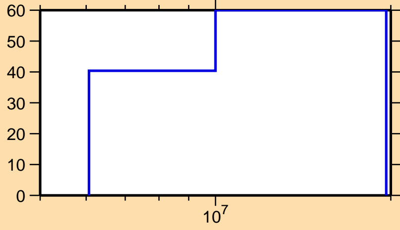
\Delta\sigma/\sigma vs. E for ^{143}\text{Cs}(n,ncont.)
