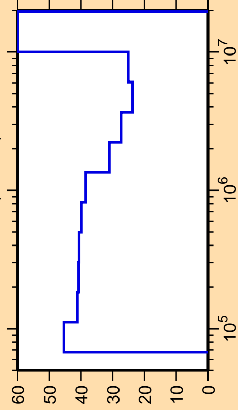
\Delta\sigma/\sigma vs. E for ^{143}\text{Cs}(n,\text{inel.})
