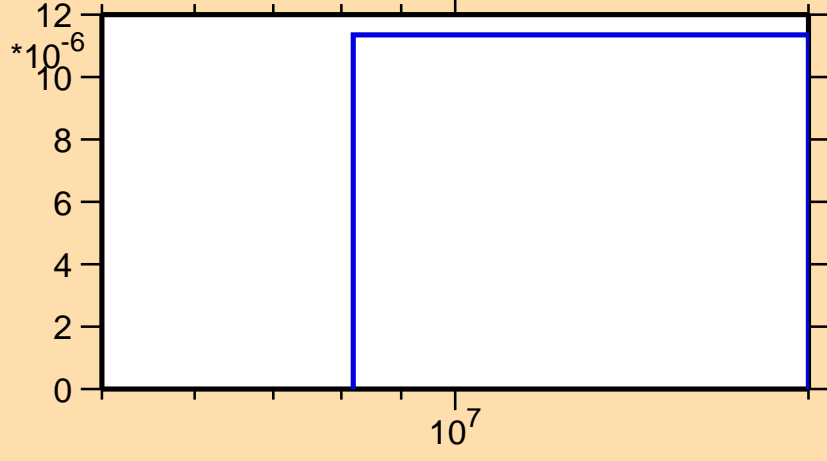
\sigma vs. E for ^{143}\text{Cs}(n,np)
