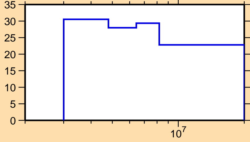
\Delta\sigma/\sigma vs. E for ^{143}\text{Cs}(n,n\text{nonel.})
