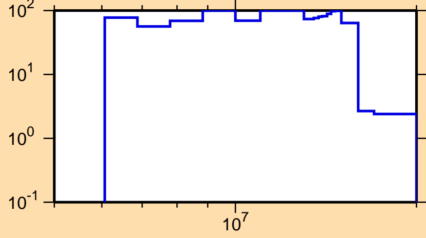
\Delta\sigma/\sigma vs. E for ^{144}\text{Cs}(n,n_1)
