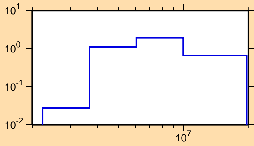
\sigma vs. E for ^{144}\text{Cs}(n,2n)
