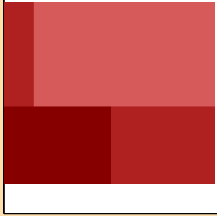
\Delta\sigma/\sigma vs. E for ^{144}\text{Cs}(n,n_1)
