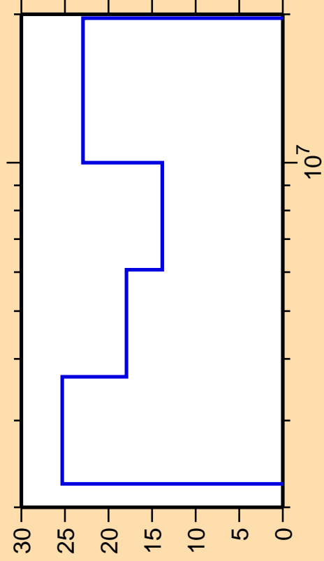
\Delta\sigma/\sigma vs. E for ^{144}\text{Cs}(n,2n)
