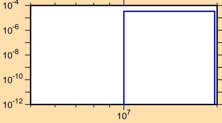
\sigma vs. E for ^{144}\text{Cs}(n,d)
