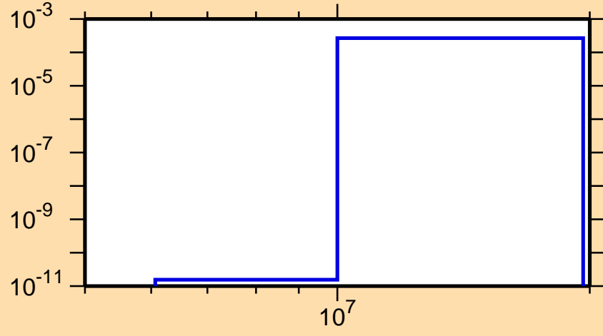
\sigma vs. E for ^{144}\text{Cs}(n,p)
