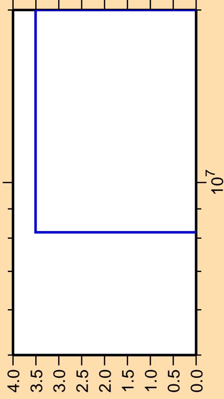
\Delta\sigma/\sigma vs. E for ^{144}\text{Cs}(\text{mt 11})
