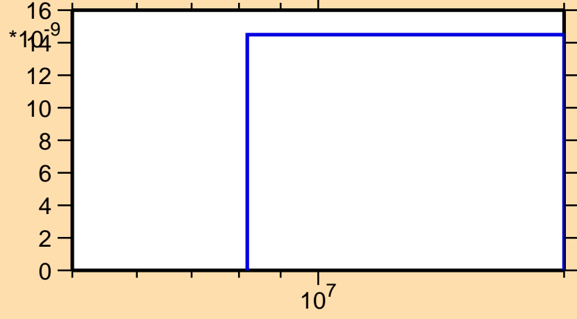
\sigma vs. E for ^{144}\text{Cs}(n,2np)
