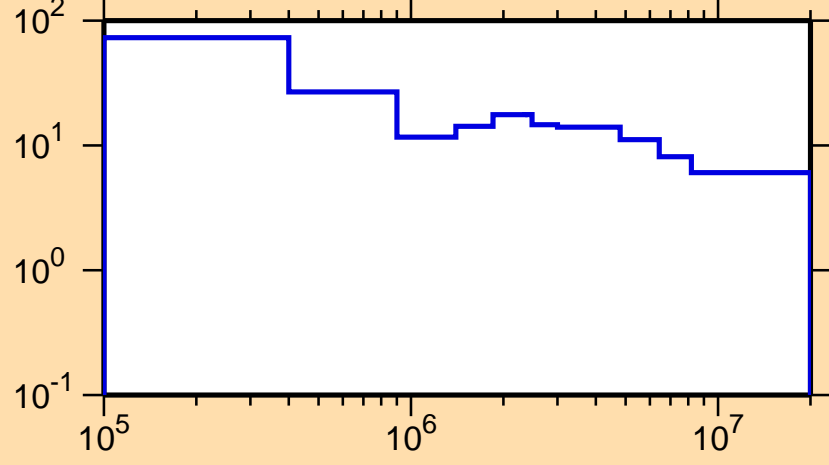
\Delta\sigma/\sigma vs. E for ^{144}\text{Cs}(n,tot.)
