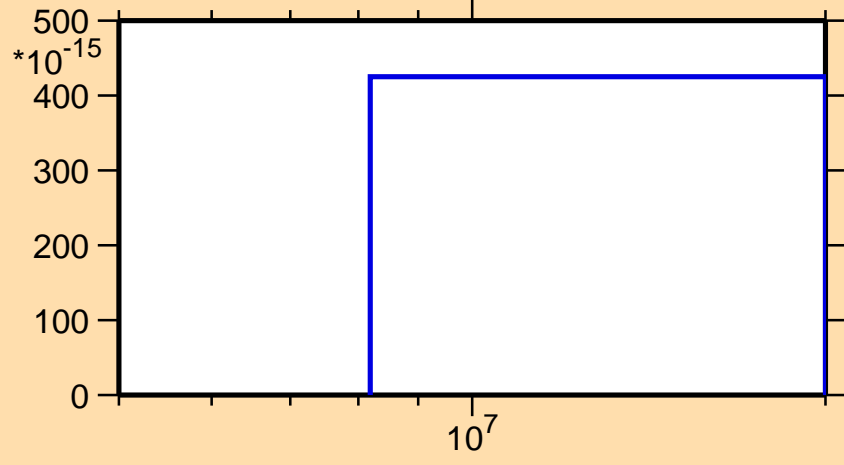
\sigma vs. E for ^{144}\text{Cs}(\text{mt 11})
