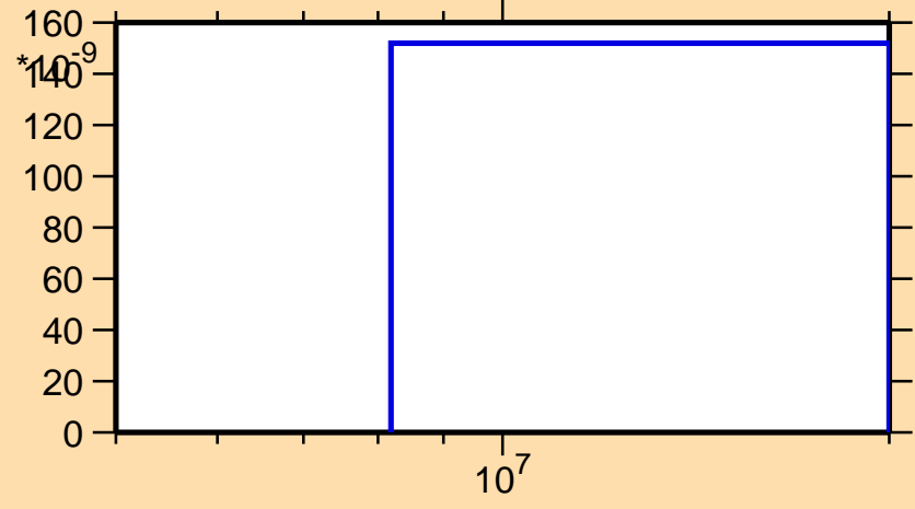
\sigma vs. E for ^{144}\text{Cs}(n,2n\alpha)
