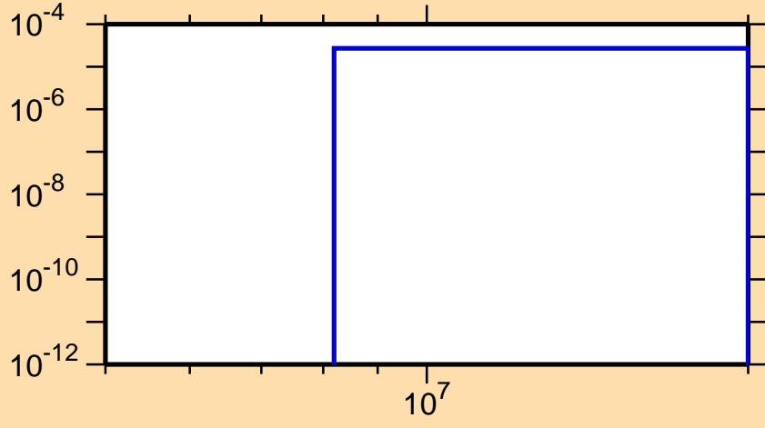
\sigma vs. E for ^{144}\text{Cs}(n,d)
