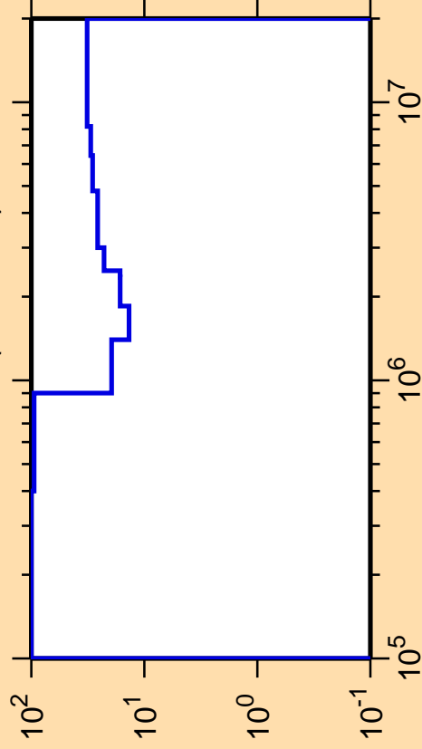
\Delta\sigma/\sigma vs. E for ^{144}\text{Cs}(n,ncont.)
