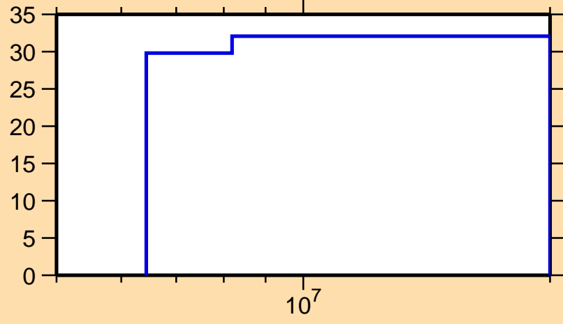
\Delta\sigma/\sigma vs. E for ^{144}\text{Cs}(n,ncont.)
