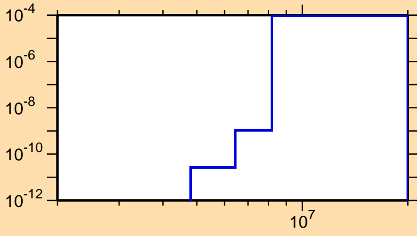
\sigma vs. E for ^{144}\text{Cs}(n,\alpha)
