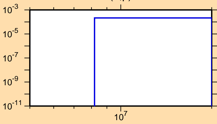
\sigma vs. E for ^{144}\text{Cs}(n,p)
