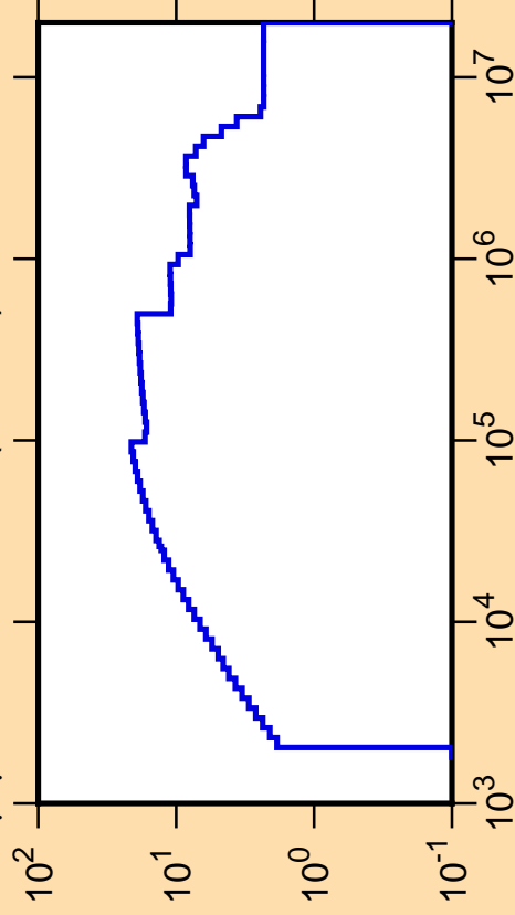
\Delta\mu/\mu vs. E for ^{58}\text{Cu}(\text{mt251})
