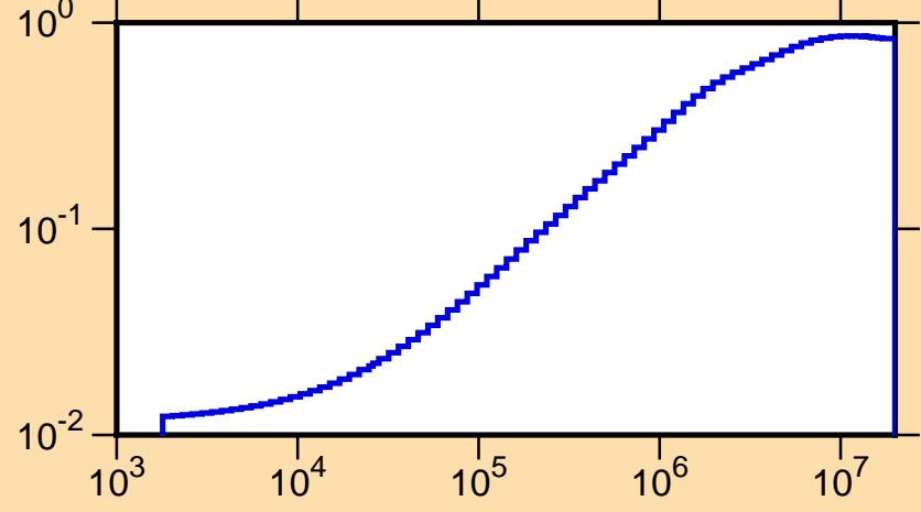
\mu vs. E for ^{58}\text{Cu}(\text{mt251})
