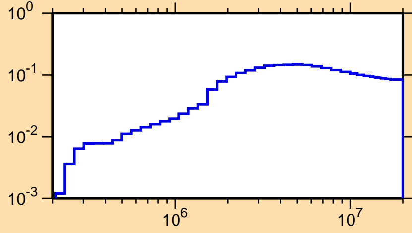
\sigma vs. E for ^{58}\text{Cu}(n,\text{inel.})
