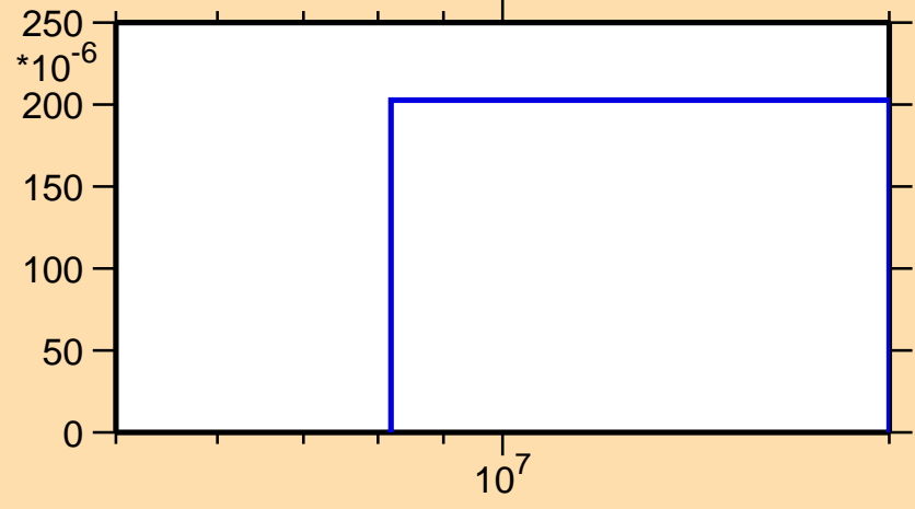
\sigma vs. E for ^{58}\text{Cu}(n,\alpha)
