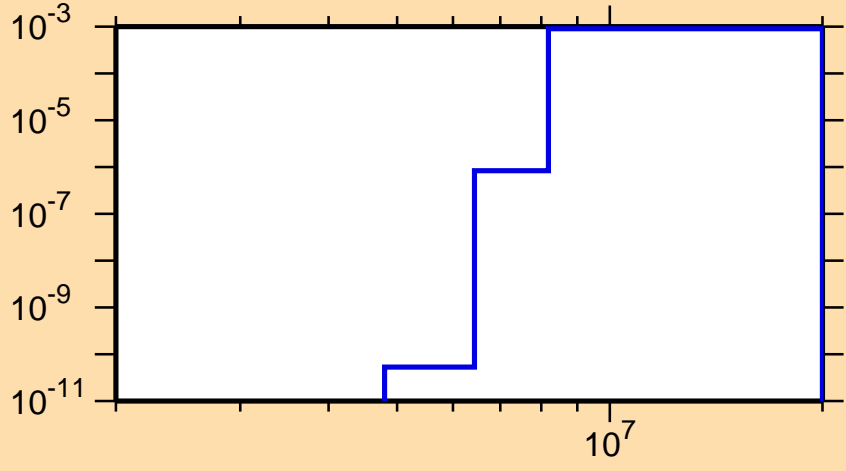
\sigma vs. E for ^{58}\text{Cu}(n,t)
