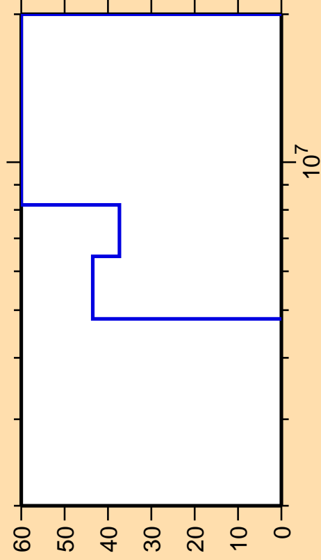
\Delta\sigma/\sigma vs. E for ^{58}\text{Cu}(n,t)
