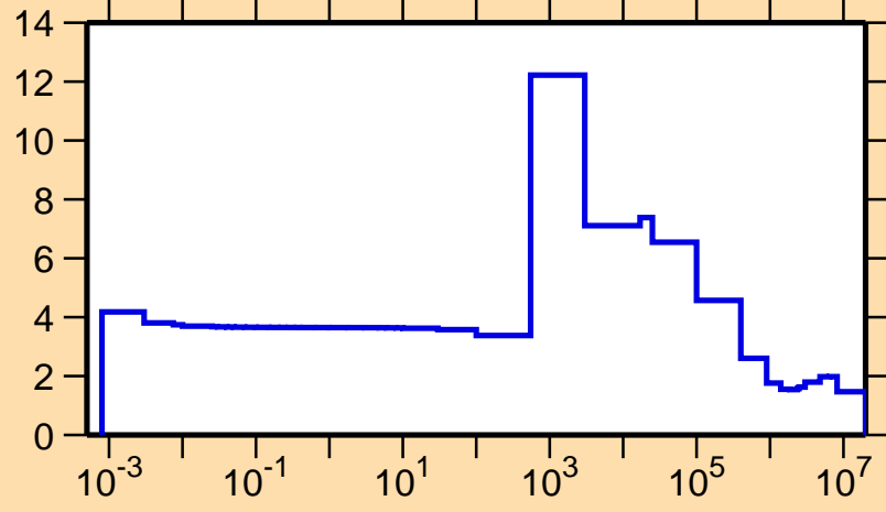
\sigma vs. E for ^{58}\text{Cu}(n,\text{el.})
