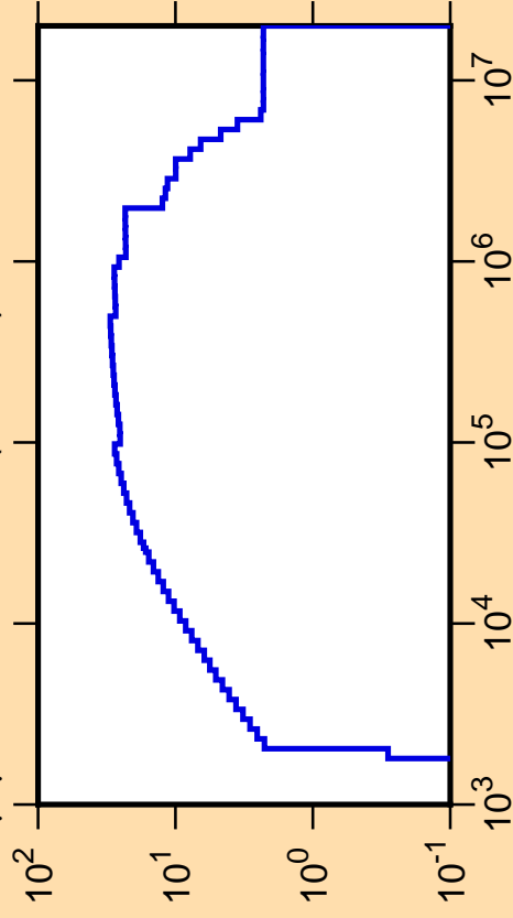
\Delta\mu/\mu vs. E for ^{59}\text{Cu}(\text{mt251})
