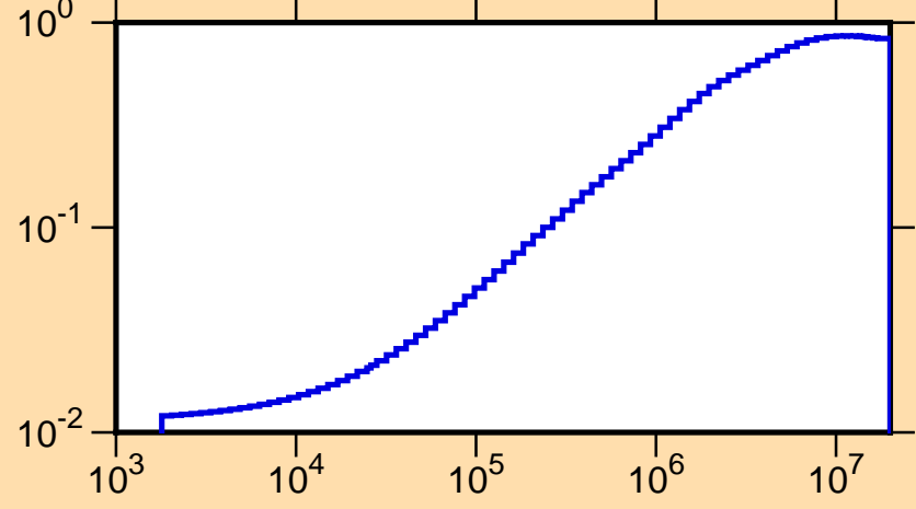
\mu vs. E for ^{59}\text{Cu}(\text{mt251})
