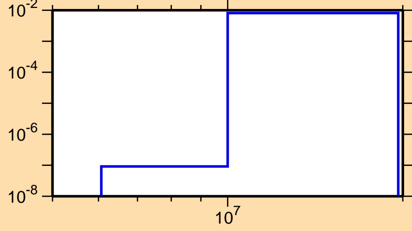
\sigma vs. E for ^{59}\text{Cu}(n,n\alpha)
