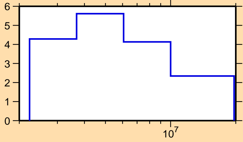
\Delta\sigma/\sigma vs. E for ^{59}\text{Cu}(n,n\text{nonel.})
