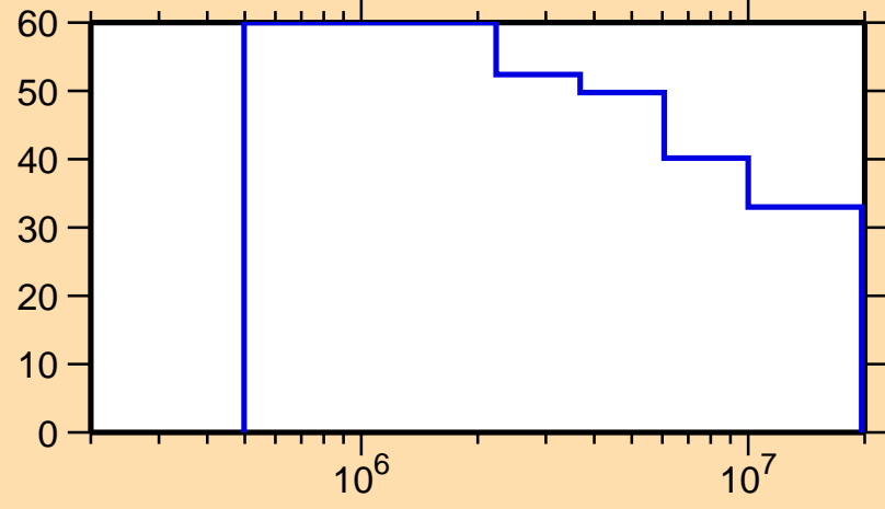
\Delta\sigma/\sigma vs. E for ^{59}\text{Cu}(n,\text{inel.})
