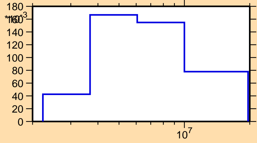
\sigma vs. E for ^{59}\text{Cu}(n,n\text{cont.})
