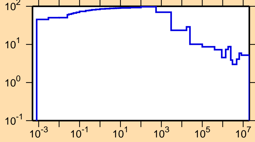
\Delta\sigma/\sigma vs. E for ^{59}\text{Cu}(n,\text{tot.})
