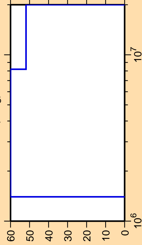
\Delta\sigma/\sigma vs. E for ^{59}\text{Cu}(n,n_3)
