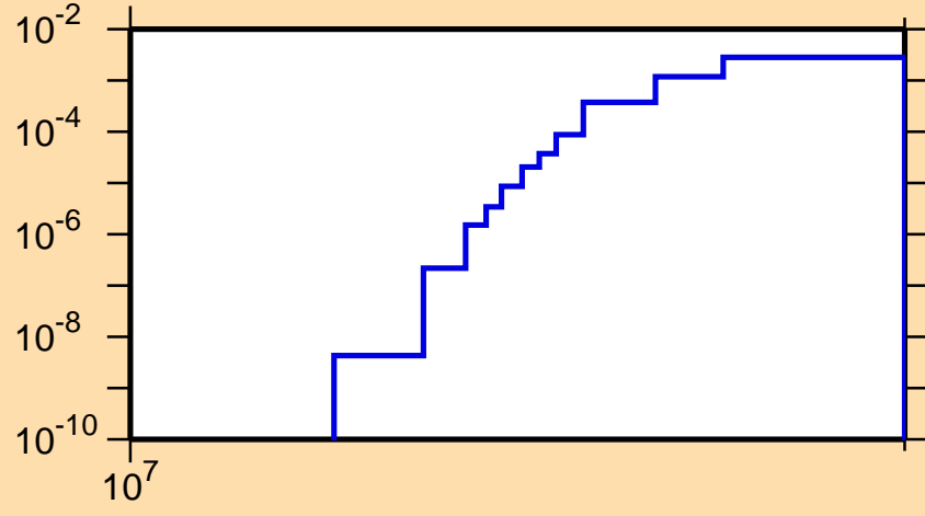
\sigma vs. E for ^{60}\text{Cu}(n,\text{nd})
