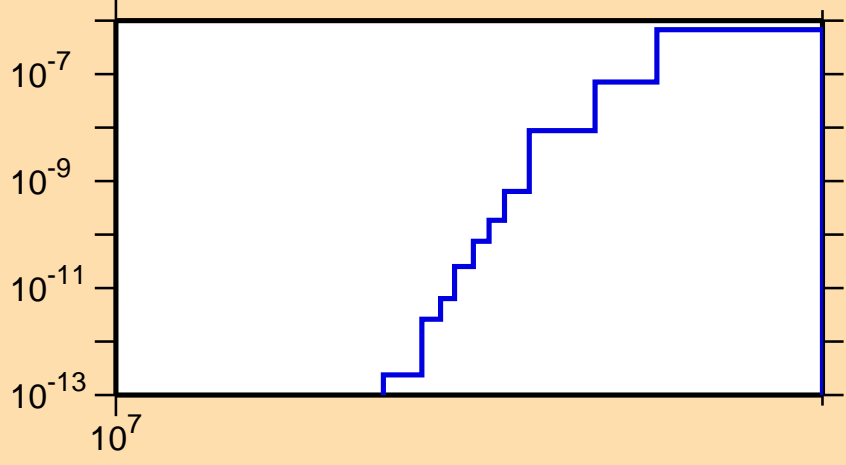
\sigma vs. E for ^{60}\text{Cu}(\text{mt117})
