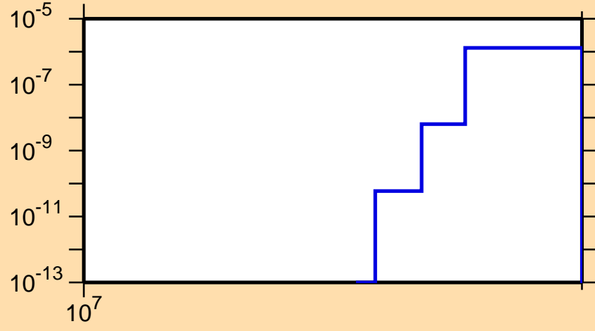
\sigma vs. E for ^{60}\text{Cu} (mt 45)
