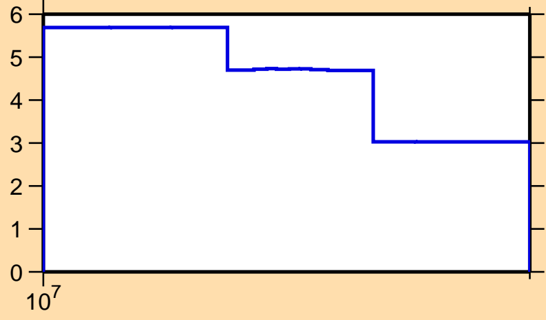
\Delta\sigma/\sigma vs. E for ^{60}\text{Cu}(n,\text{tot.})
