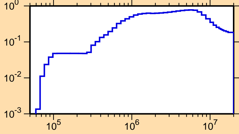
\sigma vs. E for ^{60}\text{Cu}(n,\text{inel.})
