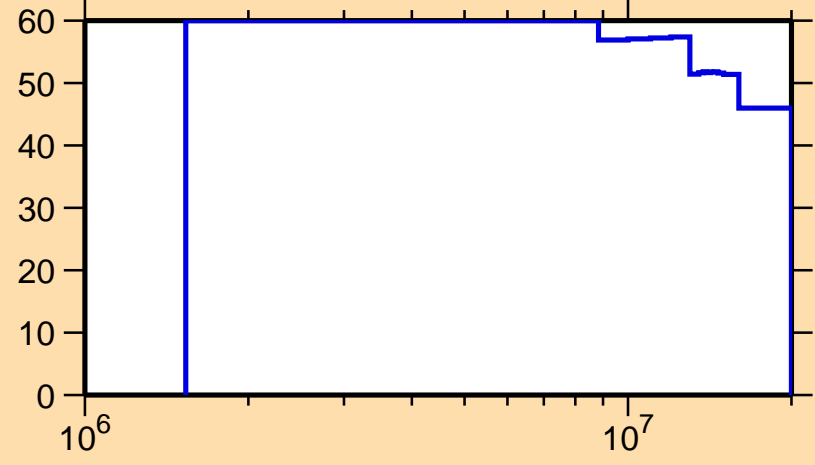
\Delta\sigma/\sigma vs. E for ^{60}\text{Cu}(n,n\text{cont.})
