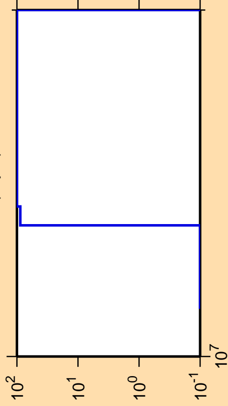
\Delta\sigma/\sigma vs. E for ^{60}\text{Cu}(n,pd)
