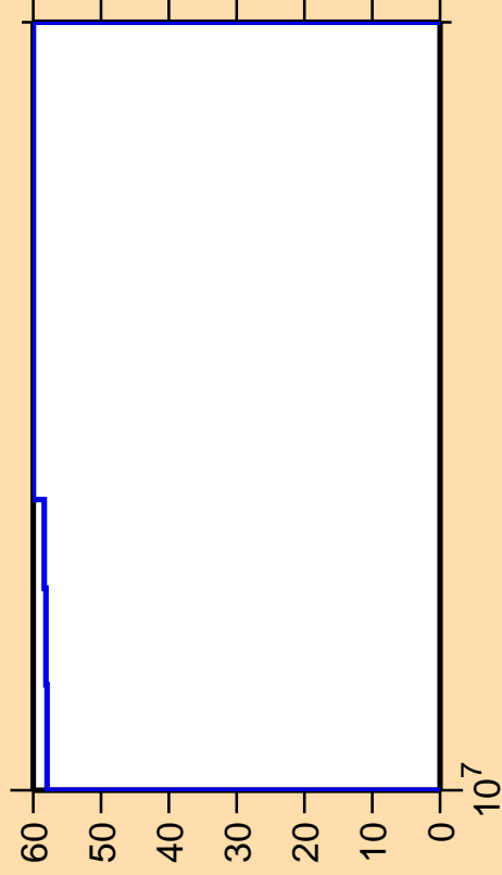
\Delta\sigma/\sigma vs. E for ^{60}\text{Cu}(n,p)
