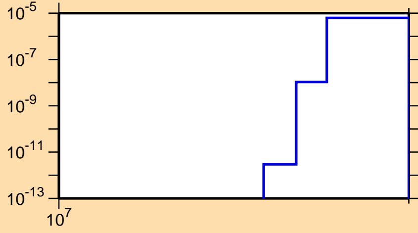
\sigma vs. E for ^{60}\text{Cu}(n,\text{pt})
