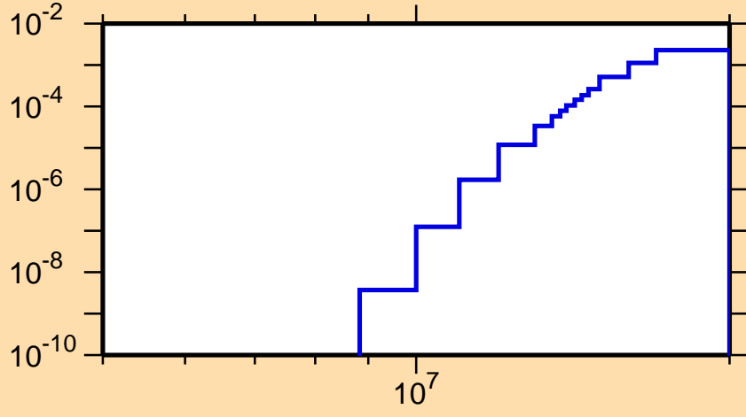
\sigma vs. E for ^{60}\text{Cu}(n,\text{He}3)
