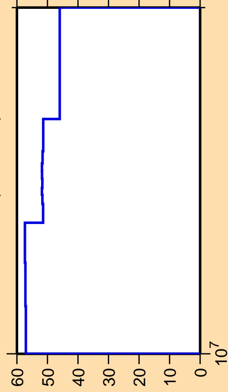
\Delta\sigma/\sigma vs. E for ^{60}\text{Cu}(n,n\text{cont.})
