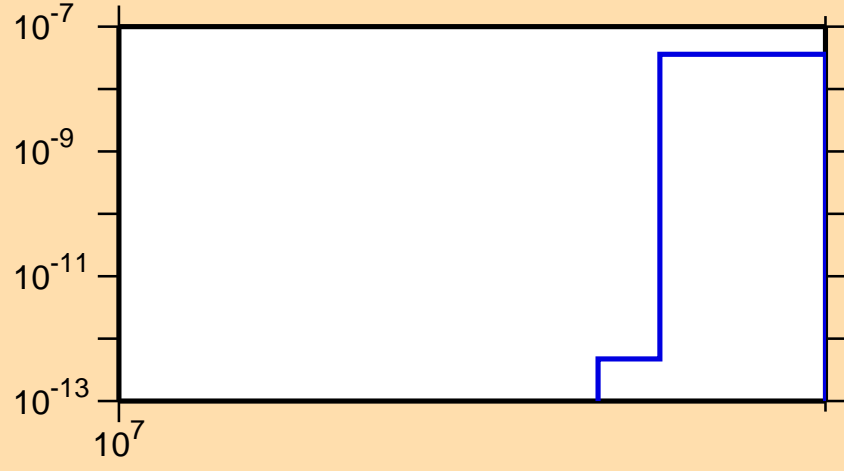
\sigma vs. E for ^{60}\text{Cu} (mt 34)
