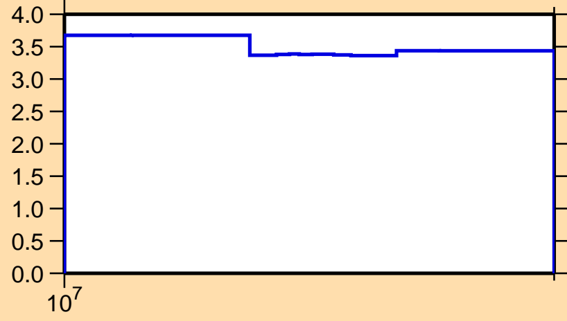
\Delta\sigma/\sigma vs. E for ^{60}\text{Cu}(n,\text{nonel.})
