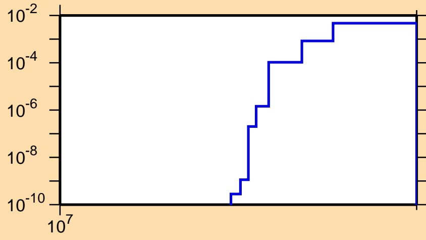
\sigma vs. E for ^{60}\text{Cu}(n,2np)
