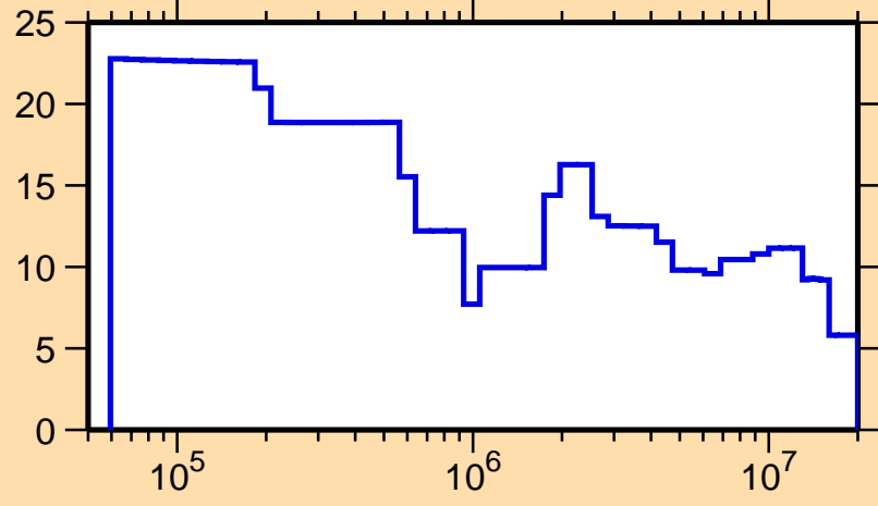
\Delta\sigma/\sigma vs. E for ^{60}\text{Cu}(n,\text{el.})
