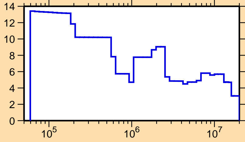
\Delta\sigma/\sigma vs. E for ^{60}\text{Cu}(n,\text{tot.})
