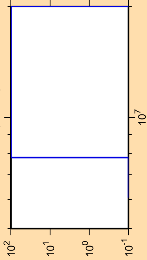
\Delta\sigma/\sigma vs. E for ^{60}\text{Cu}(n,\text{He}3)
