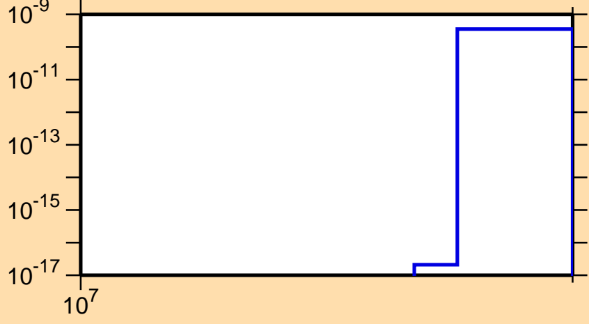
\sigma vs. E for ^{60}\text{Cu}(n,2n\alpha)
