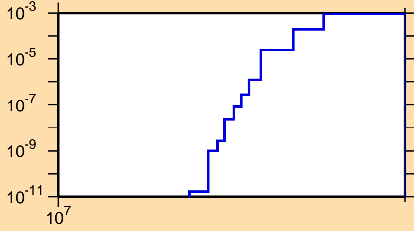
\sigma vs. E for ^{60}\text{Cu}(n,pd)
