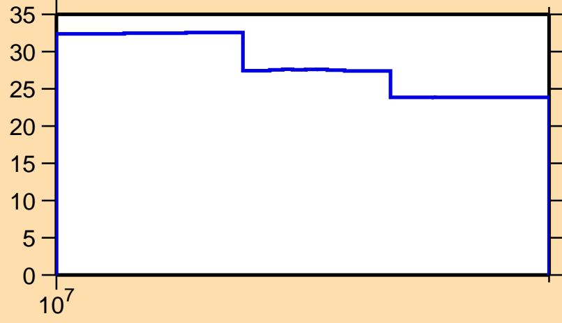
\Delta\sigma/\sigma vs. E for ^{60}\text{Cu}(n,\text{inel.})
