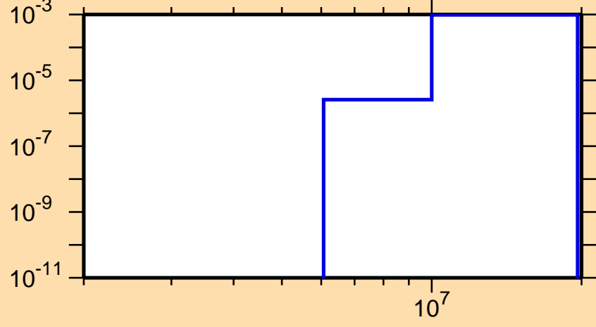
\sigma vs. E for ^{60}\text{Cu}(n,t)
