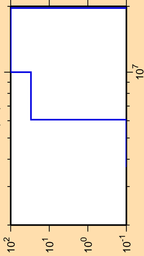
\Delta\sigma/\sigma vs. E for ^{60}\text{Cu}(n,t)
