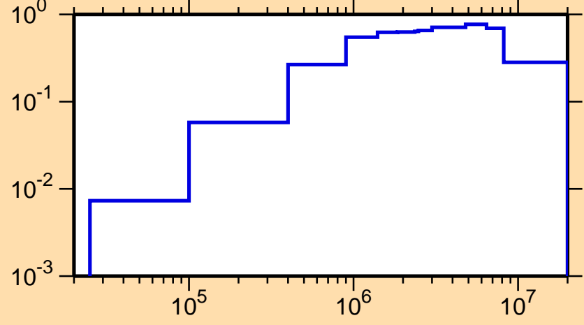
\sigma vs. E for ^{60}\text{Cu}(n,\text{inel.})
