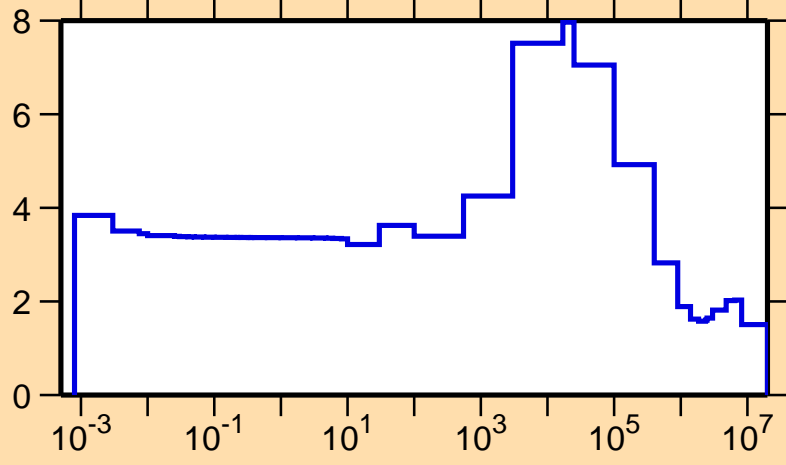
\sigma vs. E for ^{60}\text{Cu}(n,\text{el.})
