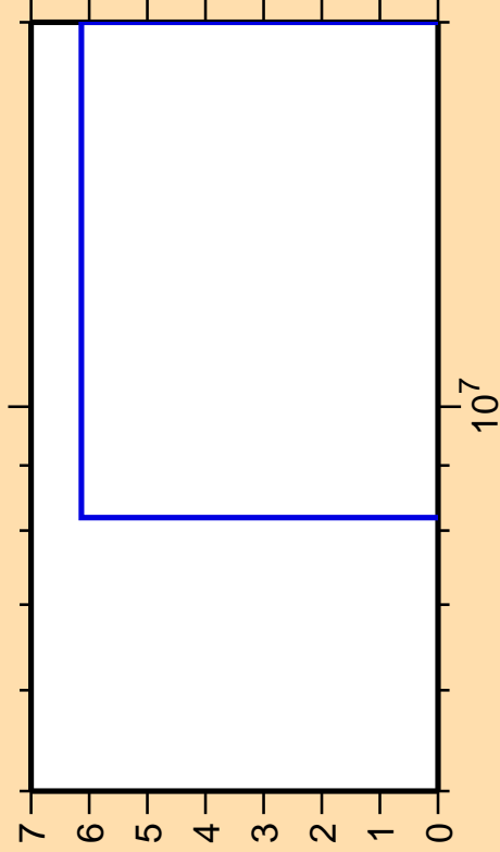
\Delta\sigma/\sigma vs. E for ^{60}\text{Cu}(n,nt)
