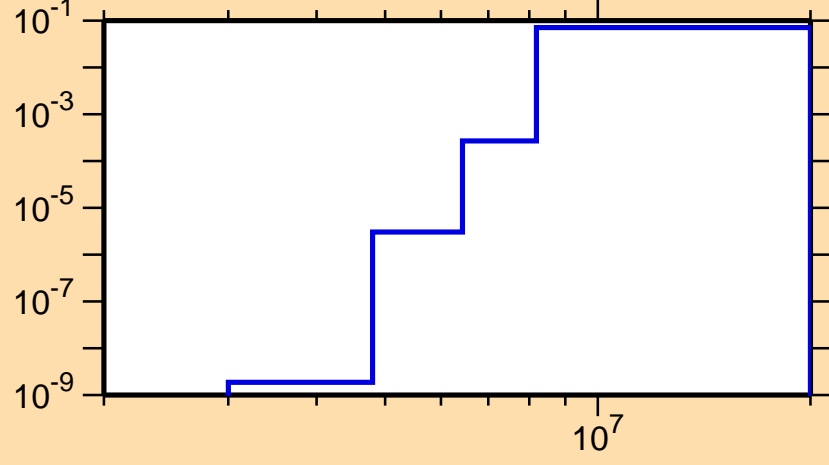
\sigma vs. E for ^{60}\text{Cu}(n,p\alpha)
