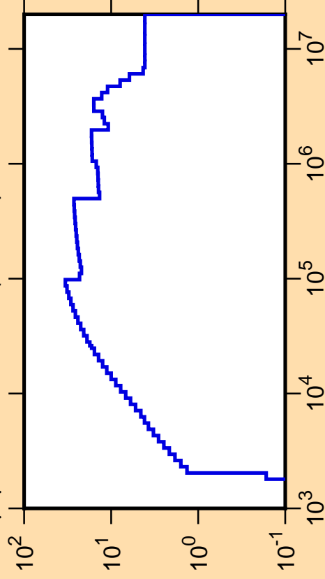
\Delta\mu/\mu vs. E for ^{61}\text{Cu}(\text{mt251})
