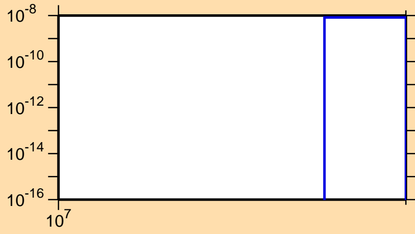
\sigma vs. E for ^{61}\text{Cu}(n,nt)
