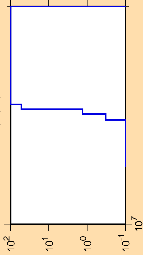
\Delta\sigma/\sigma vs. E for ^{61}\text{Cu}(n,pd)
