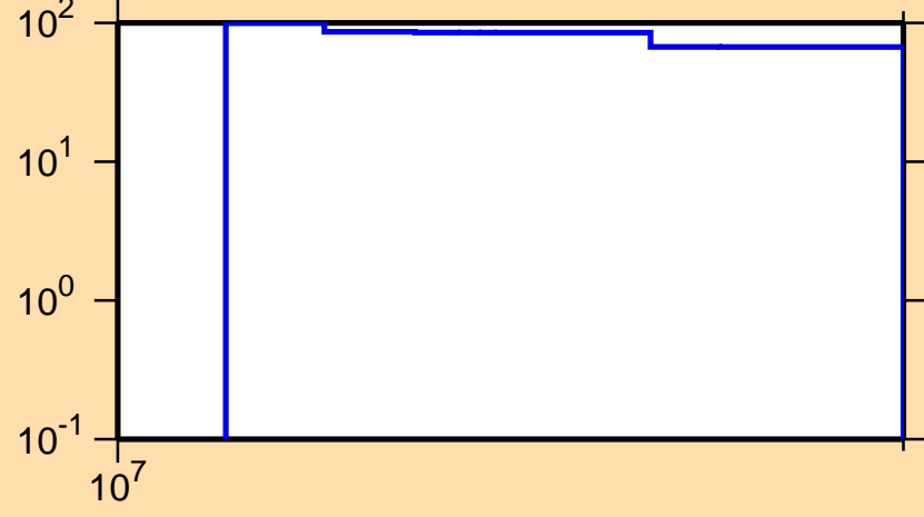
\Delta\sigma/\sigma vs. E for ^{61}\text{Cu}(n,2n)
