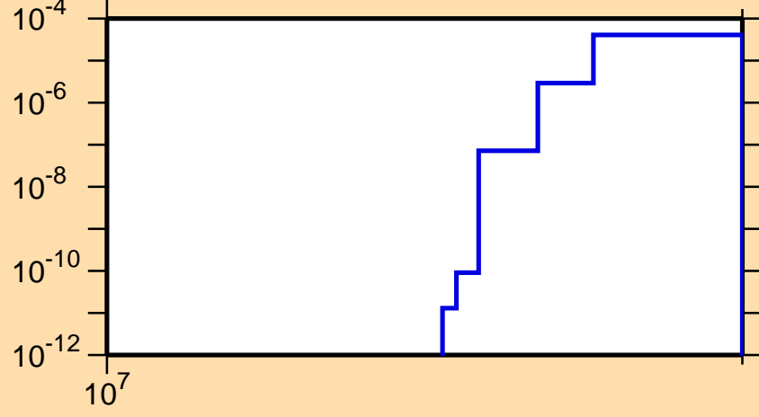
\sigma vs. E for ^{61}\text{Cu}(n,pd)
