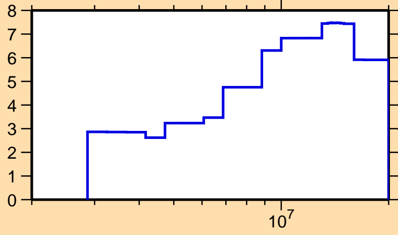
\Delta\sigma/\sigma vs. E for ^{61}\text{Cu}(n,tot.)
