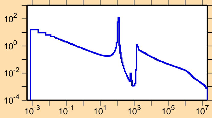
\sigma vs. E for ^{61}\text{Cu}(n,\gamma)
