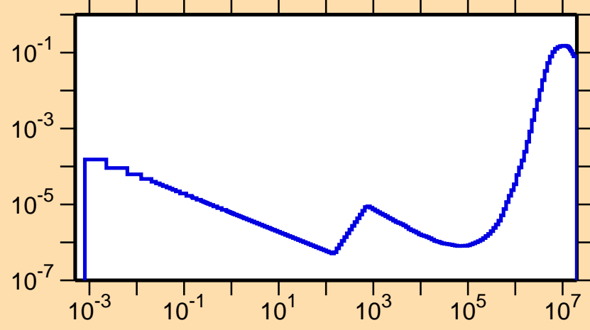
\sigma vs. E for ^{61}\text{Cu}(n,\alpha)
