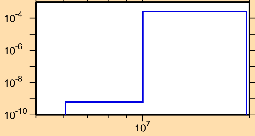
\sigma vs. E for ^{61}\text{Cu}(n,t)
