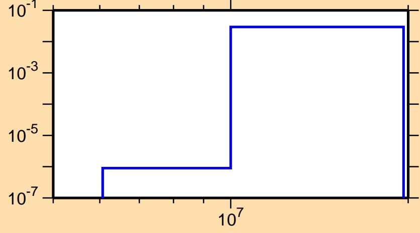
\sigma vs. E for ^{61}\text{Cu}(n,n\alpha)
