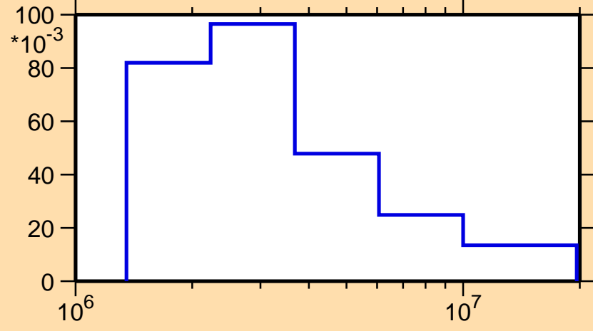
\sigma vs. E for ^{61}\text{Cu}(n,n_4)
