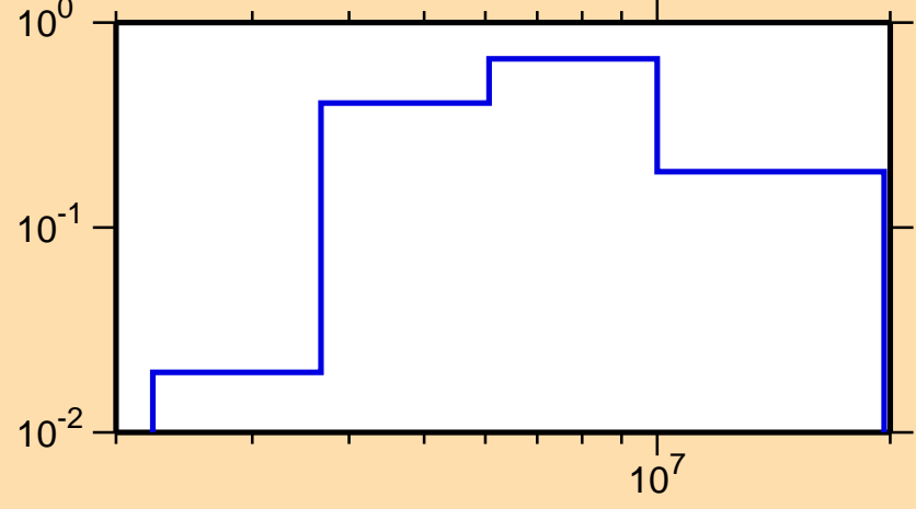
\sigma vs. E for ^{61}\text{Cu}(n,n\text{cont.})
