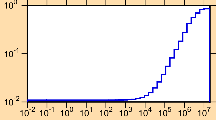
\mu vs. E for ^{62}\text{Cu}(\text{mt251})
