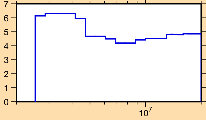
\Delta\sigma/\sigma vs. E for ^{63}\text{Cu}(n,n\text{onel.})
