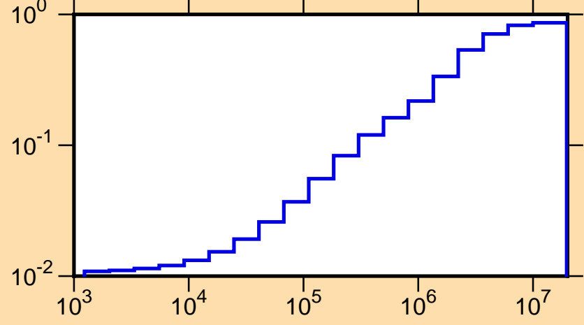
\mu vs. E for ^{63}\text{Cu}(\text{mt251})
