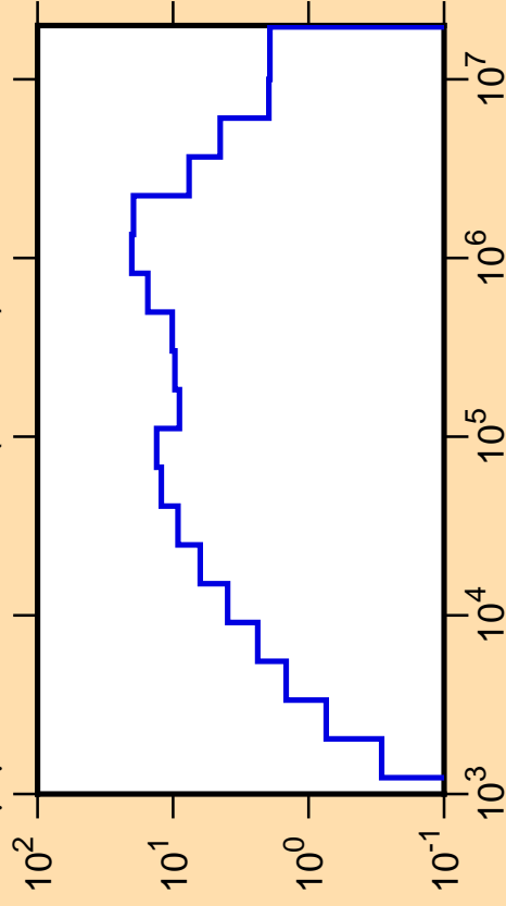
\Delta\mu/\mu vs. E for ^{63}\text{Cu}(\text{mt251})
