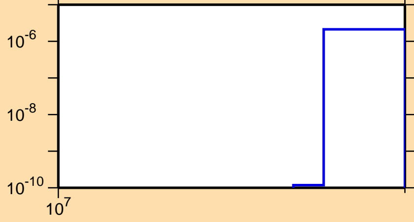
\sigma vs. E for ^{64}\text{Cu}(n,2n\alpha)
