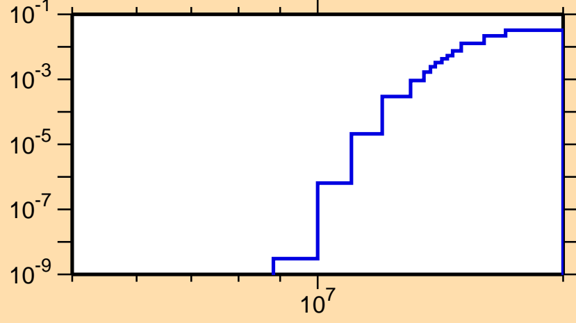
\sigma vs. E for ^{64}\text{Cu}(n,n\alpha)
