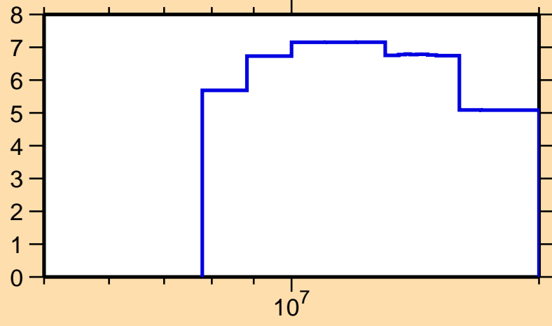
\Delta\sigma/\sigma vs. E for ^{64}\text{Cu}(n,\text{tot.})
