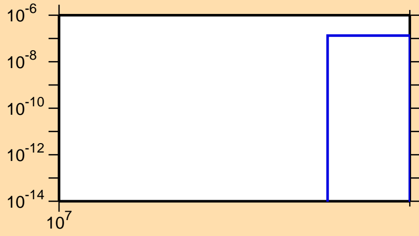
\sigma vs. E for ^{64}\text{Cu}(n,nt)
