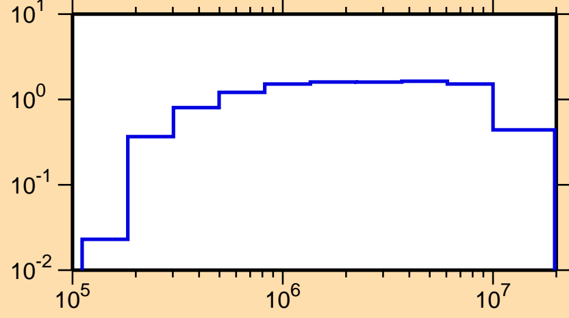
\sigma vs. E for ^{64}\text{Cu}(n,\text{inel.})
