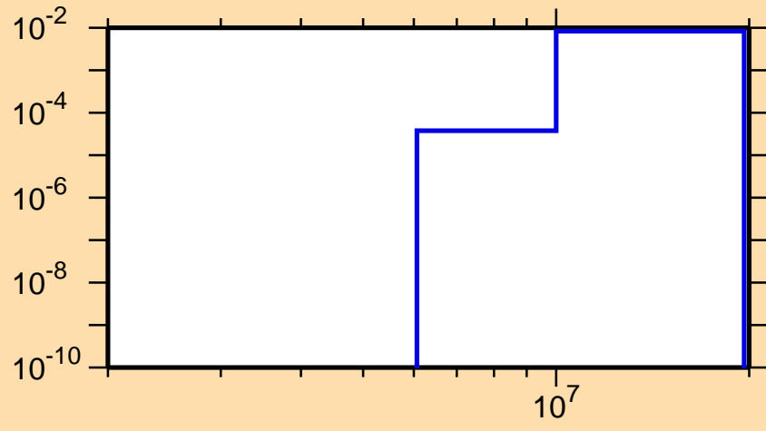
\sigma vs. E for ^{64}\text{Cu}(n,d)
