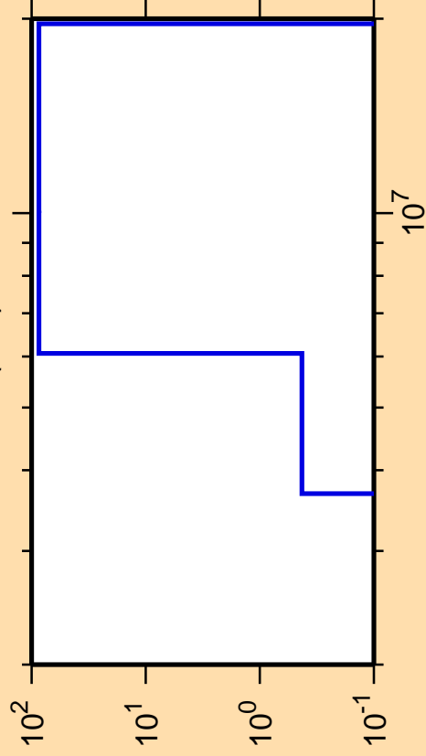
\Delta\sigma/\sigma vs. E for ^{64}\text{Cu}(n,d)
