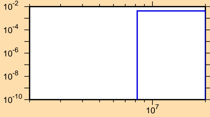
\sigma vs. E for ^{64}\text{Cu}(n,\alpha)
