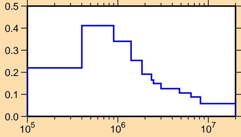
\sigma vs. E for ^{64}\text{Cu}(n,n_1)
