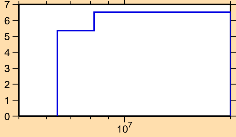
\Delta\sigma/\sigma vs. E for ^{64}\text{Cu}(n,\text{tot.})
