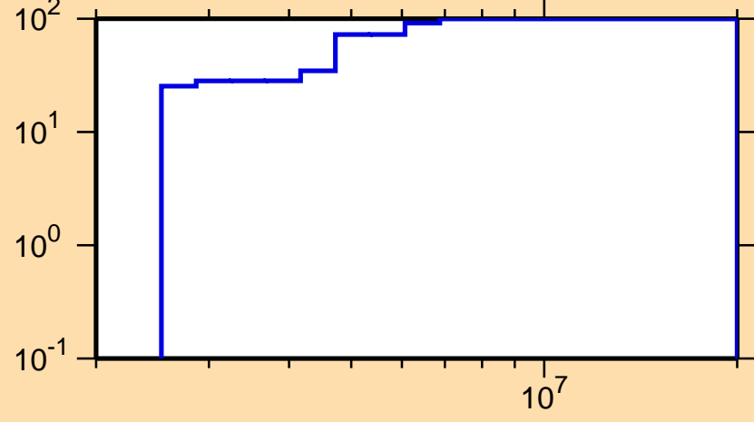
\Delta\sigma/\sigma vs. E for ^{65}\text{Cu}(n,\gamma)
