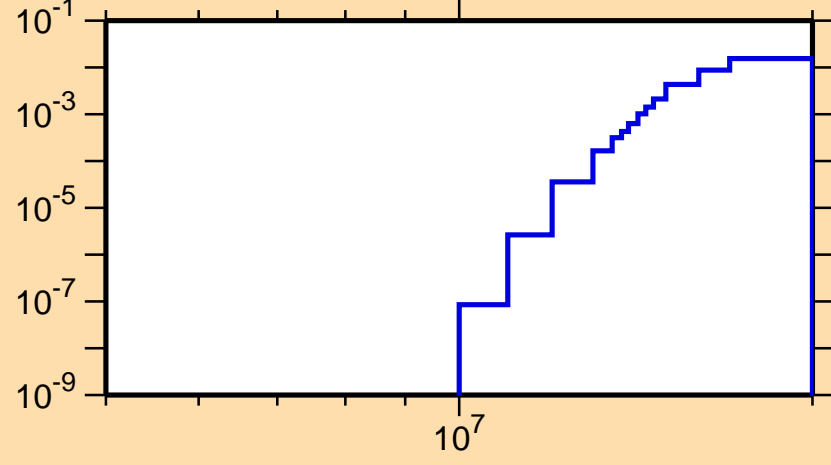
\sigma vs. E for ^{65}\text{Cu}(n,\alpha)
