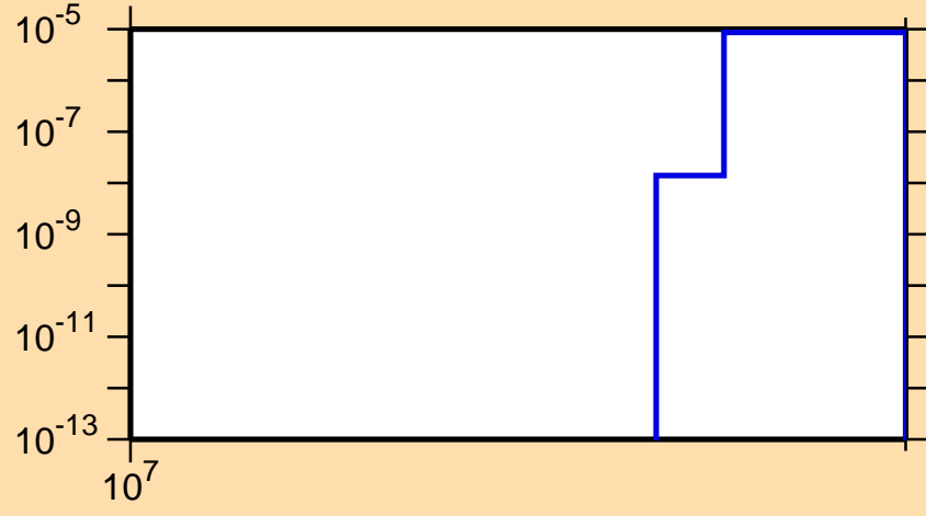
\sigma vs. E for ^{65}\text{Cu}(n,\text{nd})
