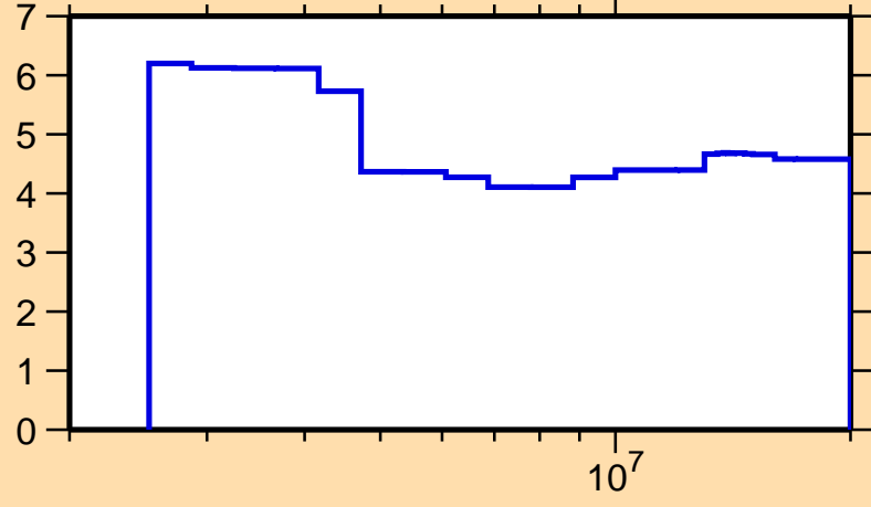
\Delta\sigma/\sigma vs. E for ^{65}\text{Cu}(n,\text{nonel.})
