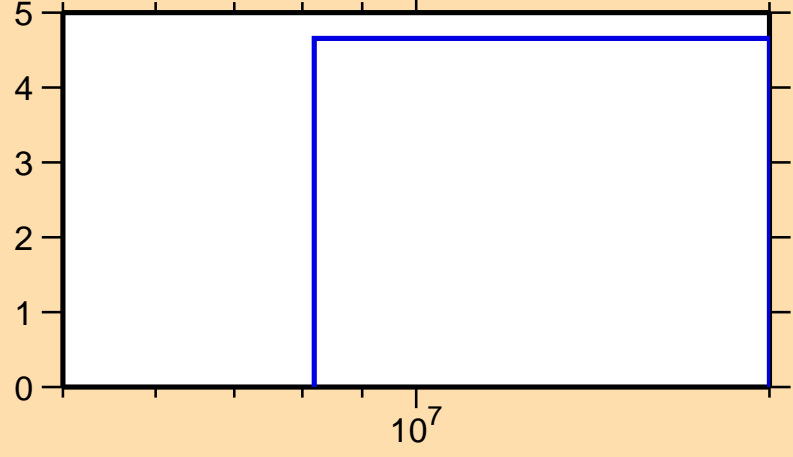
\Delta\sigma/\sigma vs. E for ^{65}\text{Cu}(n,\text{tot.})
