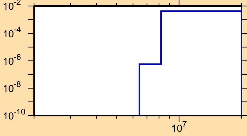
\sigma vs. E for ^{65}\text{Cu}(n,d)
