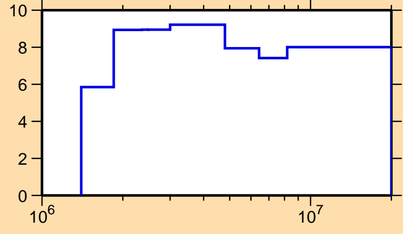
\Delta\sigma/\sigma vs. E for ^{65}\text{Cu}(n,el.)
