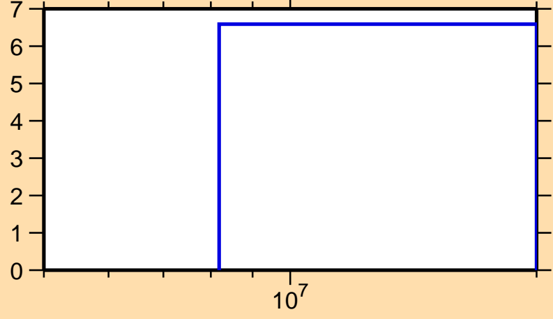
\Delta\sigma/\sigma vs. E for ^{65}\text{Cu}(n,2n)
