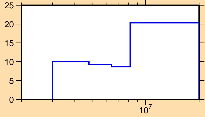
\Delta\sigma/\sigma vs. E for ^{65}\text{Cu}(n,ncont.)
