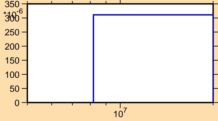
\sigma vs. E for ^{65}\text{Cu}(n,t)
