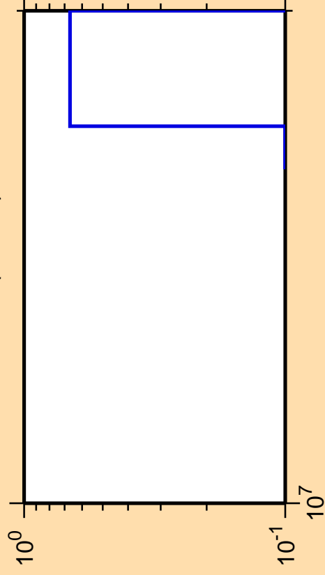
\Delta\sigma/\sigma vs. E for ^{67}\text{Cu}(n,2n\alpha)
