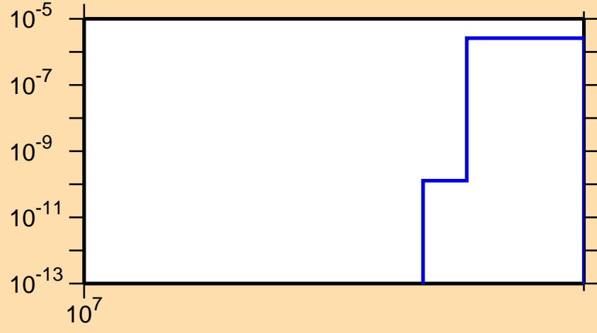
\sigma vs. E for ^{67}\text{Cu}(n,\text{nd})
