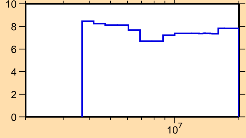
\Delta\sigma/\sigma vs. E for ^{67}\text{Cu}(n,n\text{inel.})
