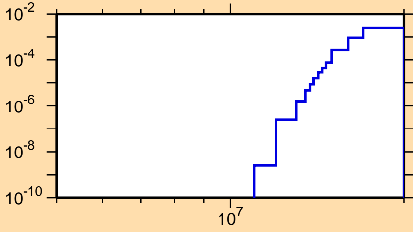
\sigma vs. E for ^{67}\text{Cu}(n,\alpha)
