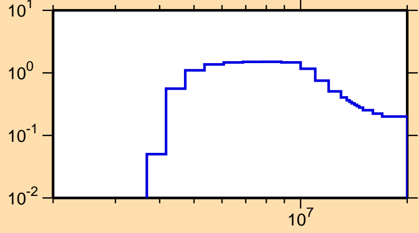
\sigma vs. E for ^{67}\text{Cu}(n,n\text{cont.})
