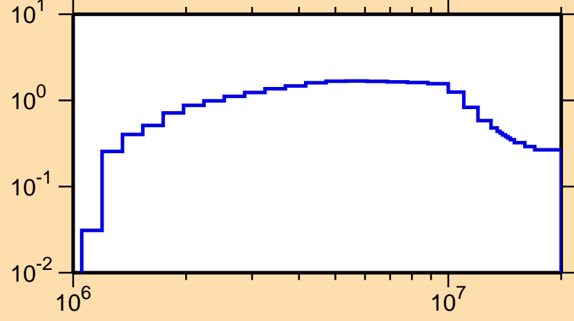
\sigma vs. E for ^{67}\text{Cu}(n,\text{inel.})
