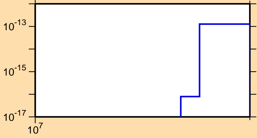
\sigma vs. E for ^{67}\text{Cu}(n,2n\alpha)
