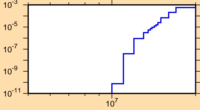
\sigma vs. E for ^{67}\text{Cu}(n,t)
