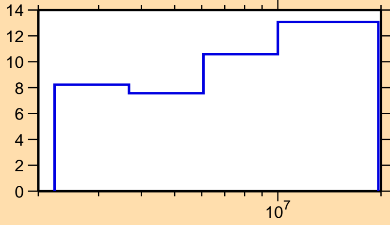
\Delta\sigma/\sigma vs. E for ^{67}\text{Cu}(n,el.)
