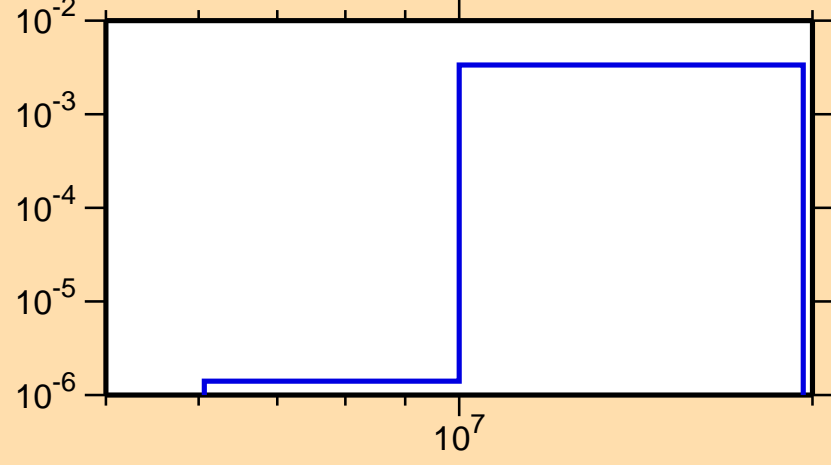
\sigma vs. E for ^{67}\text{Cu}(n,d)
