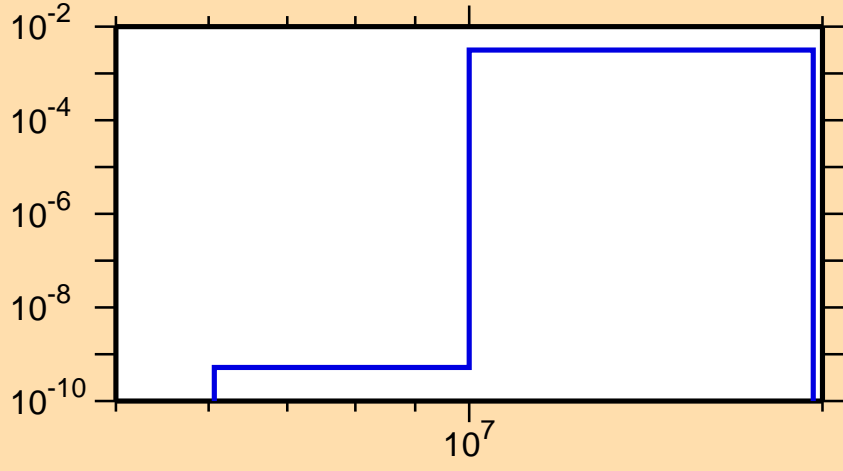
\sigma vs. E for ^{67}\text{Cu}(n,np)
