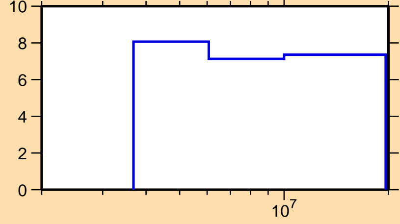
\Delta\sigma/\sigma vs. E for ^{67}\text{Cu}(n,n\text{onel.})
