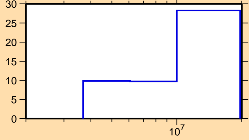
\Delta\sigma/\sigma vs. E for ^{67}\text{Cu}(n,ncont.)
