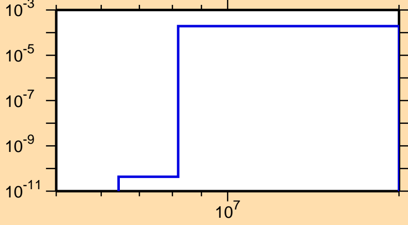
\sigma vs. E for ^{68}\text{Cu}(n,t)
