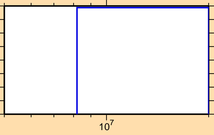
\sigma vs. E for ^{68}\text{Cu}(n,2np)
