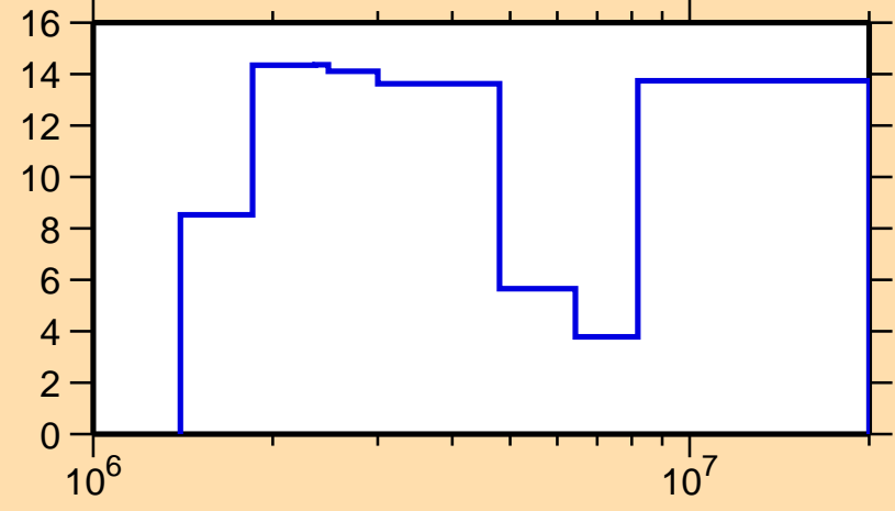
\Delta\sigma/\sigma vs. E for ^{68}\text{Cu}(n,el.)
