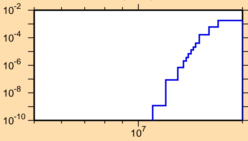
\sigma vs. E for ^{68}\text{Cu}(n,\alpha)
