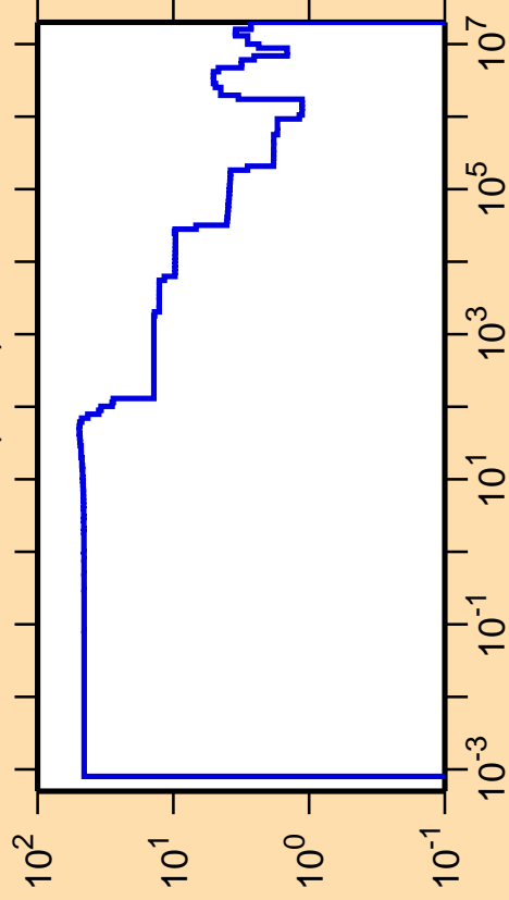
\Delta\sigma/\sigma vs. E for ^{68}\text{Cu}(n,\text{el.})
