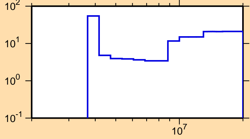
\Delta\sigma/\sigma vs. E for ^{69}\text{Cu}(n,n\text{cont.})
