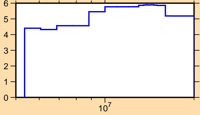
\Delta\sigma/\sigma vs. E for ^{69}\text{Cu}(n,\text{el.})
