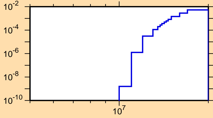
\sigma vs. E for ^{69}\text{Cu}(n,np)
