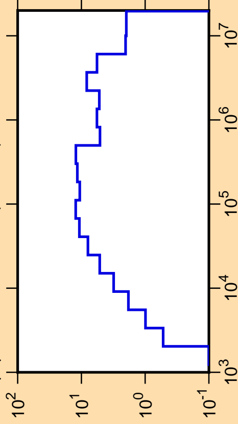
\Delta\mu/\mu vs. E for ^{69}\text{Cu}(\text{mt251})
