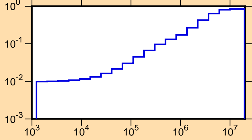
\mu vs. E for ^{69}\text{Cu}(\text{mt251})
