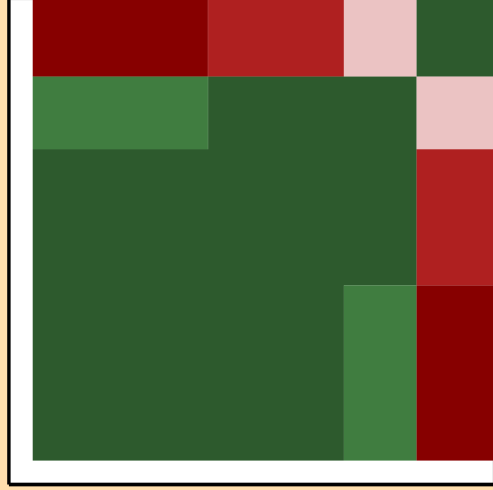
\sigma vs. E for ^{70}\text{Cu}(n,2n)
