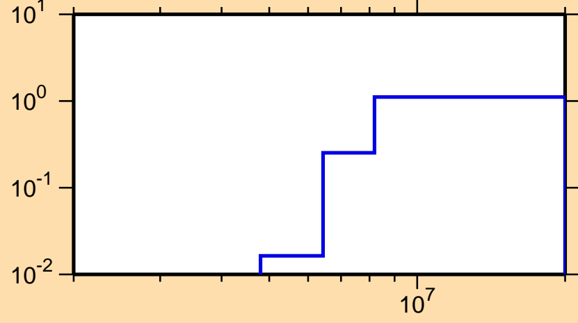
\sigma vs. E for ^{70}\text{Cu}(n,2n)
