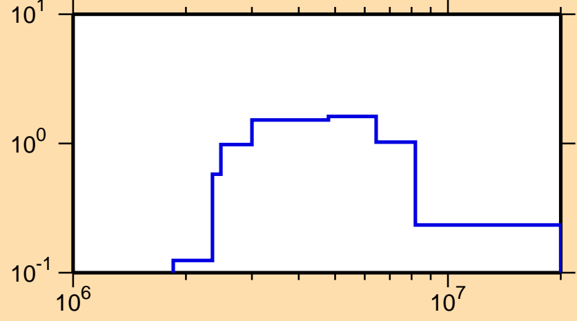
\sigma vs. E for ^{70}\text{Cu}(n,n\text{cont.})
